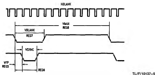
FIGURE 2A. Vertical Waveform Specification
