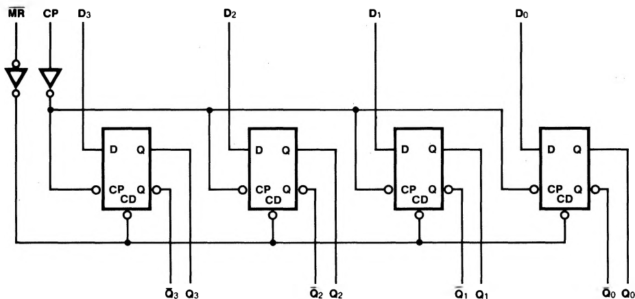
LOGIC DIAGRAM
