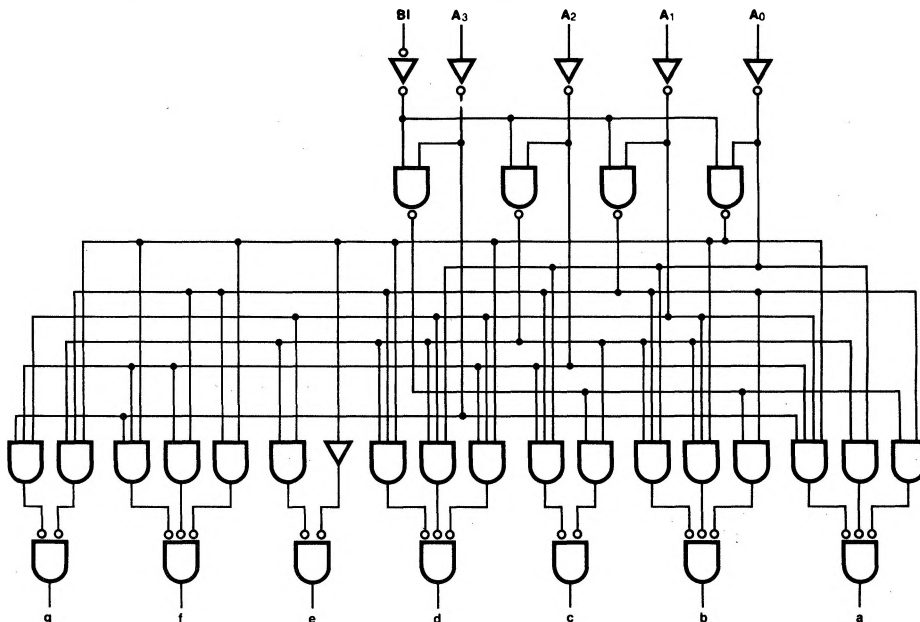
LOGIC DIAGRAM
