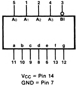
LOGIC SYMBOL
