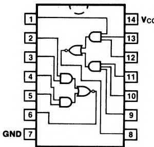
PINOUT B
