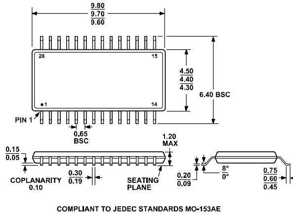
Figure 57. 28-Lead Thin Shrink Small Outline Package [TSSOP] (RU-28)—Dimensions shown in millimeters
