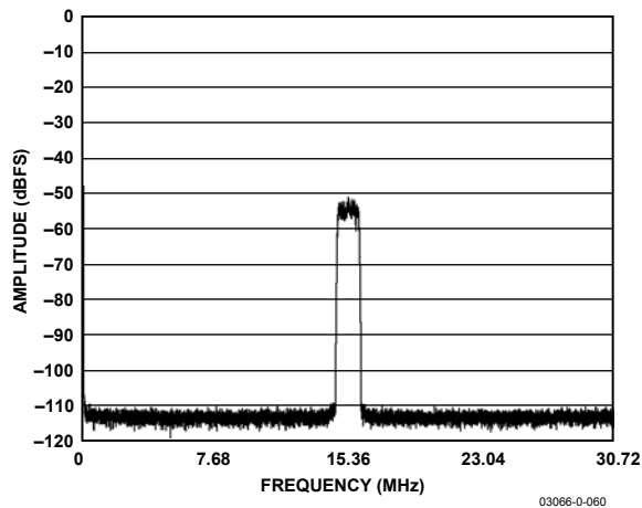
Figure 23. 32K FFT CDMA2K Carrier @ F_{IN} = 46.08 MHz: Sample Rate = 61.44 MSPS
