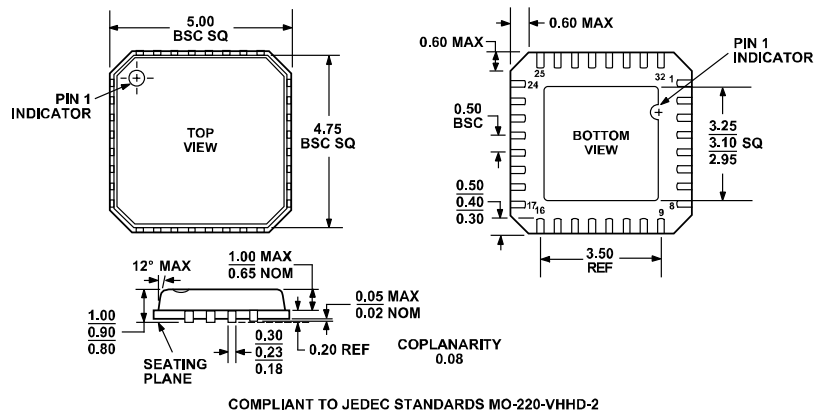
Figure 58. 32-Lead Frame Chip Scale Package [LFCSF] (CP-32)—Dimensions shown in millimeters
