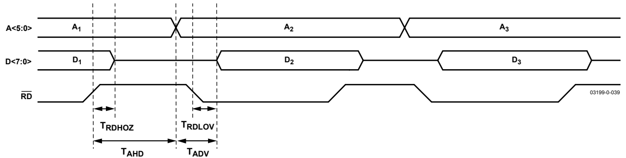
Figure 34. I/O Port Write Cycle Timing (Parallel)
