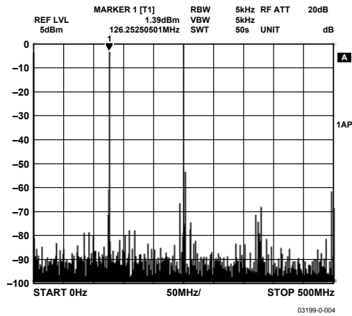
Figure 4. Wideband SFDR, 126 MHz F_{OUT}
