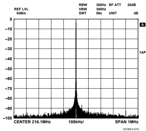
Figure 9. Narrow-Band SFDR, 201 MHz F_{OUT} , 1 MHz BW, 1 GHz Clock, Divider Off
