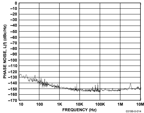
Figure 14. Residual Phase Noise, 103 MHz F_{OUT} , 1 GHz REFCLK
