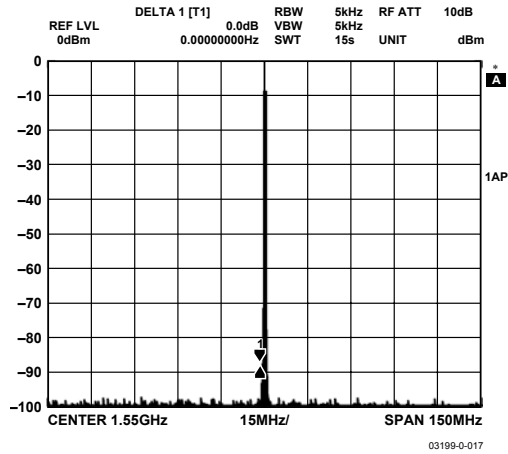
Figure 20. Fractional Divider Loop SFDR, F_{IN} = 96.9 MHz, F_{OUT} = 1550 MHz, BW = 150 MHz
