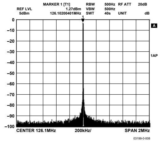
Figure 7. Narrow-Band SFDR, 126 MHz F_{OUT} , 1 MHz BW
