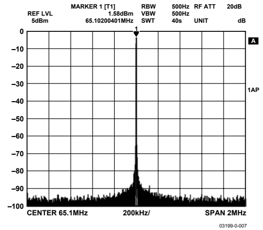
Figure 6. Narrow-Band SFDR, 65 MHz F_{OUT} , 1 MHz BW
