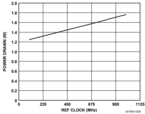
Figure 26. Supply Current vs. REFCLK ( F_{OUT} = REFCLK/5 )
