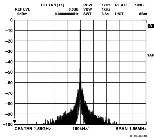
Figure 16. Fractional Divider Loop SFDR, F_{IN} = 96.9 MHz, F_{OUT} = 1550 MHz, BW = 1.5 MHz
