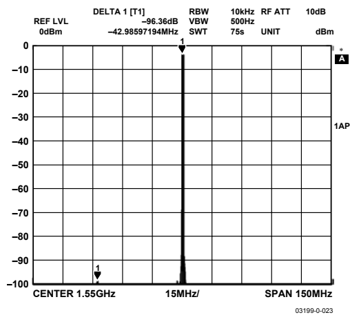
Figure 22. Translation Loop SFDR, F_{LO} = 1459 MHz, F_{OUT} = 1550 MHz, BW = 150 MHz
