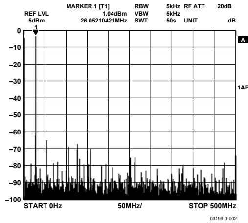
Figure 2. Wideband SFDR, 26 MHz F_{OUT}
