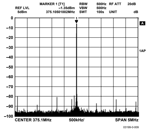
Figure 11. Narrow-Band SFDR, 375 MHz F_{OUT} , 1 MHz BW
