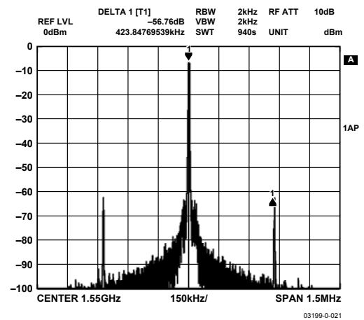
Figure 19. Fractional Divider Loop SFDR, F_{IN} = 97.3 MHz, F_{OUT} = 1550 MHz, BW = 1.5 MHz
