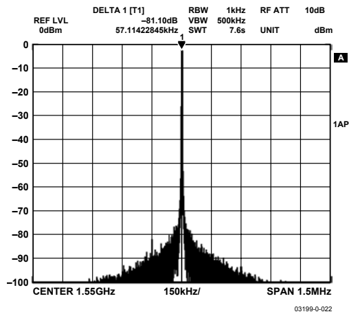
Figure 21. Translation Loop SFDR, F_{LO} = 1459 MHz, F_{OUT} = 1550 MHz, BW = 1.5 MHz
