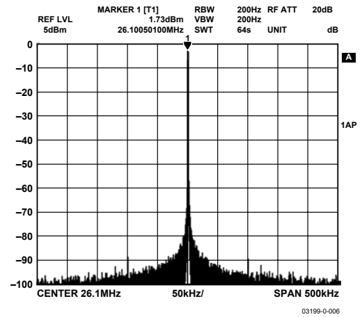
Figure 5. Narrow-Band SFDR, 26 MHz F_{OUT} , 1 MHz BW
