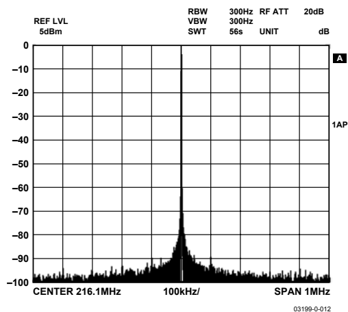
Figure 10. Narrow-Band SFDR, 201 MHz F_{OUT} , 1 MHz BW, 2 GHz Clock, Divider On
