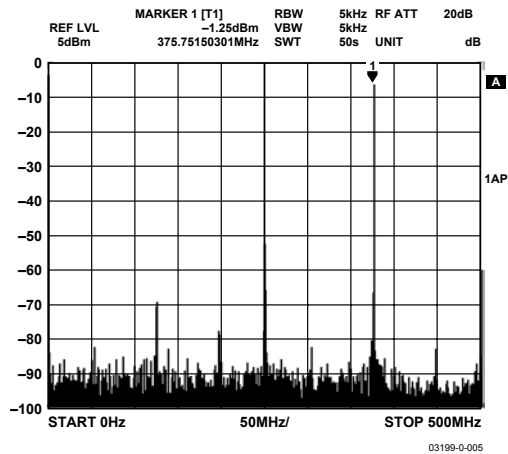
Figure 8. Wideband SFDR, 375 MHz F_{OUT}
