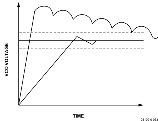
Figure 29. Symbolic Representation of Charge Pump to Loop Filter Connection
