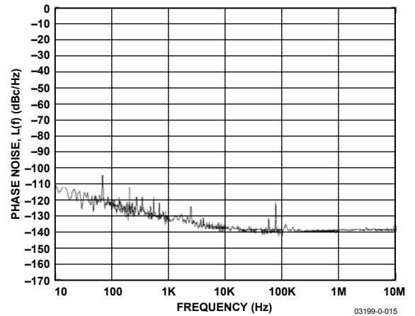
Figure 17. Residual Phase Noise, 403 MHz F_{OUT} , 1 GHz REFCLK
