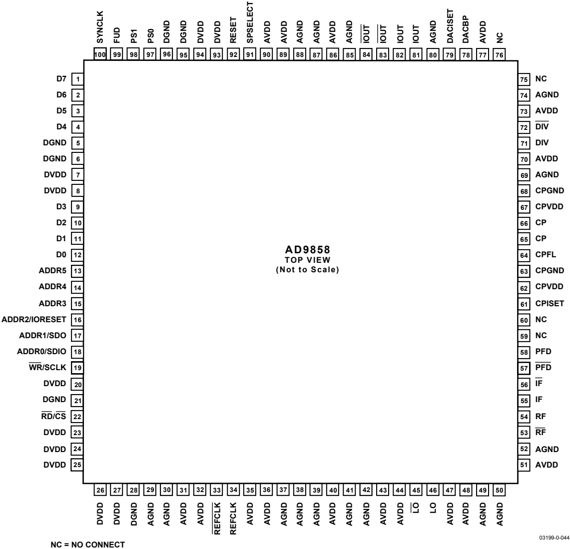
Figure 39. 100-Lead EPAD (SV-100)
