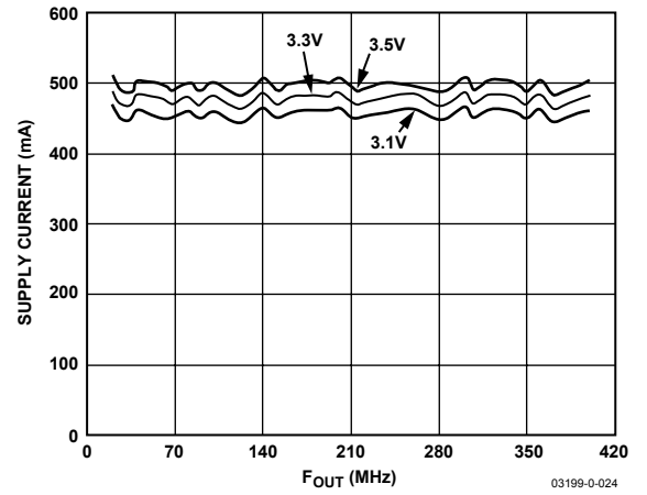
Figure 27. Supply Current vs. F_{OUT} (1 GHz REFCLK)
