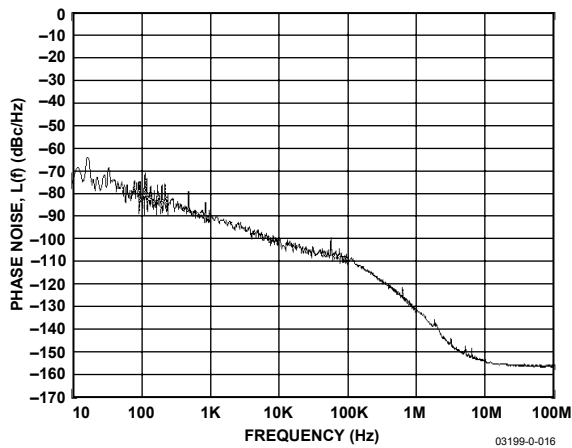
Figure 15. Fractional Divider Loop Residual Phase Noise, F_{IN} = 115 MHz, F_{OUT} = 1550 MHz, Loop BW = 50 kHz
