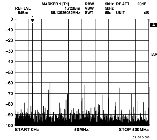
Figure 3. Wideband SFDR, 65 MHz F_{OUT}
