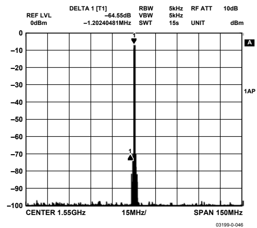
Figure 25. Translation Loop SFDR, F_{LO} = 1410 MHz, F_{OUT} = 1550 MHz, BW = 150 MHz
