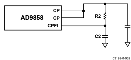
Figure 28. Symbolic Representation of Charge Pump to Loop Filter Connection
