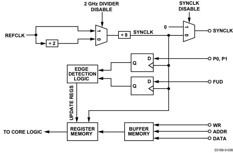
Figure 32. I/O Synchronization Block Diagram
