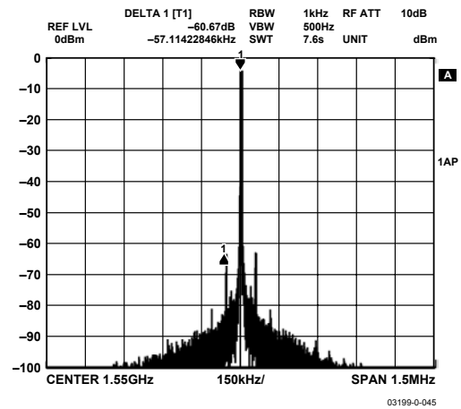
Figure 24. Translation Loop SFDR, F_{LO} = 1410 MHz, F_{OUT} = 1550 MHz, BW = 1.5 MHz
