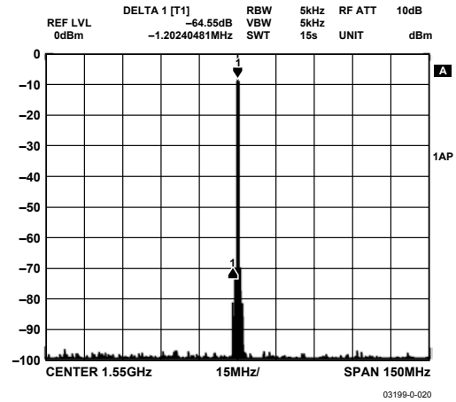
Figure 23. Fractional Divider Loop SFDR, F_{IN} = 97.3 MHz, F_{OUT} = 1550 MHz, BW = 150 MHz
