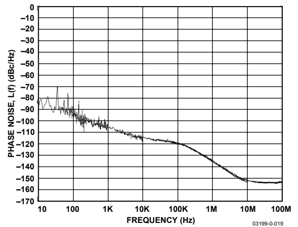
Figure 18. Translation Loop Residual Phase Noise F_{LO} = 1500 MHz, F_{OUT} = 1550 MHz Loop BW = 50 kHz
