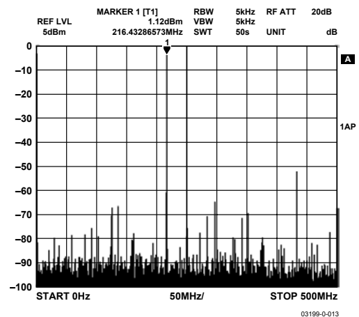
Figure 13. Wideband SFDR, 201 MHz F_{OUT} , 2 GHz Clock, Divider On
