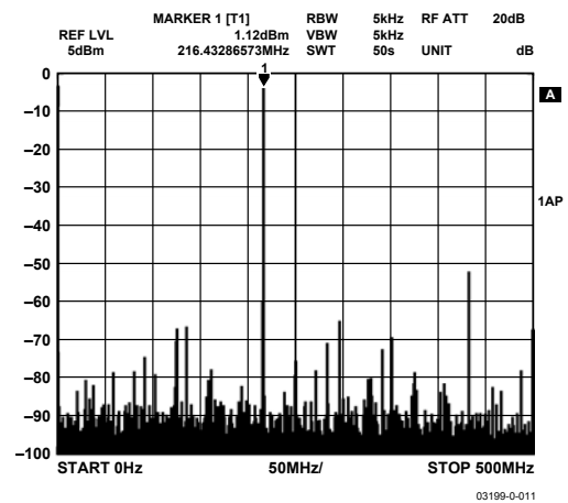
Figure 12. Wideband SFDR, 201 MHz F_{OUT} , 1 GHz Clock, Divider Off
