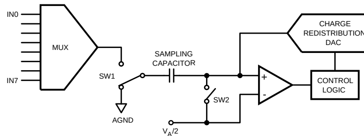
Figure 5. ADC088S102 in Hold Mode
