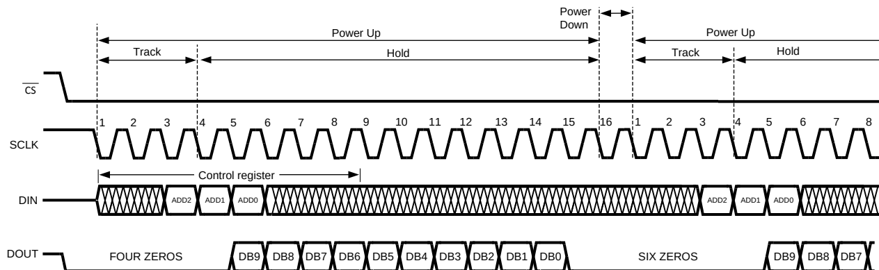
Figure 1. ADC088S102 Operational Timing Diagram
