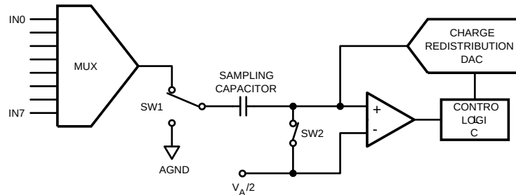
Figure 4. ADC088S102 in Track Mode
