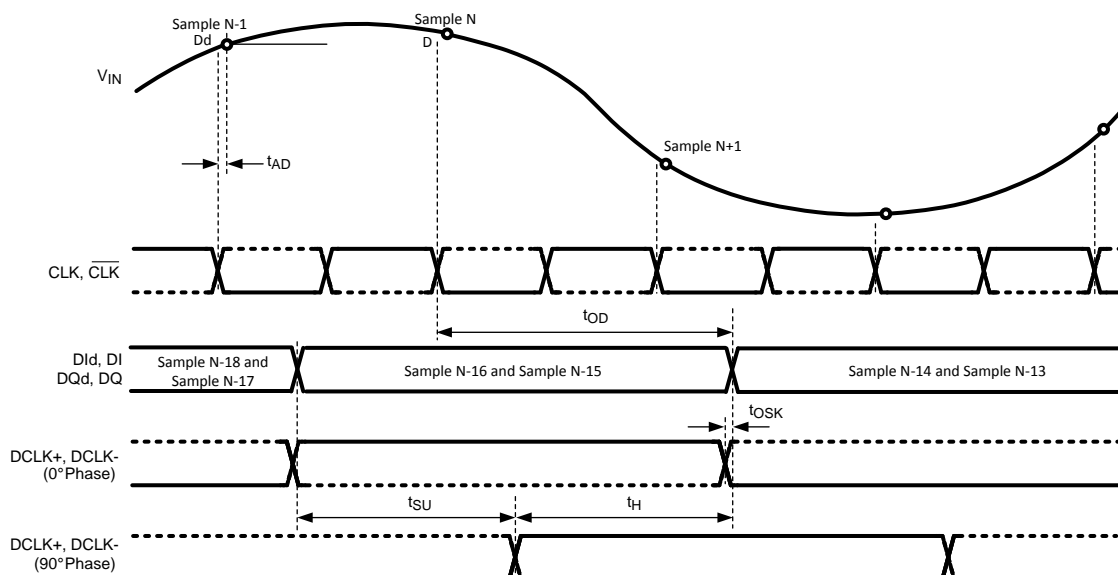
Figure 5. ADC08D1020 Timing — DDR Clocking in 1:2 Demultiplexed and Normal Mode
