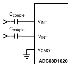
Figure 43. Differential Input Drive
