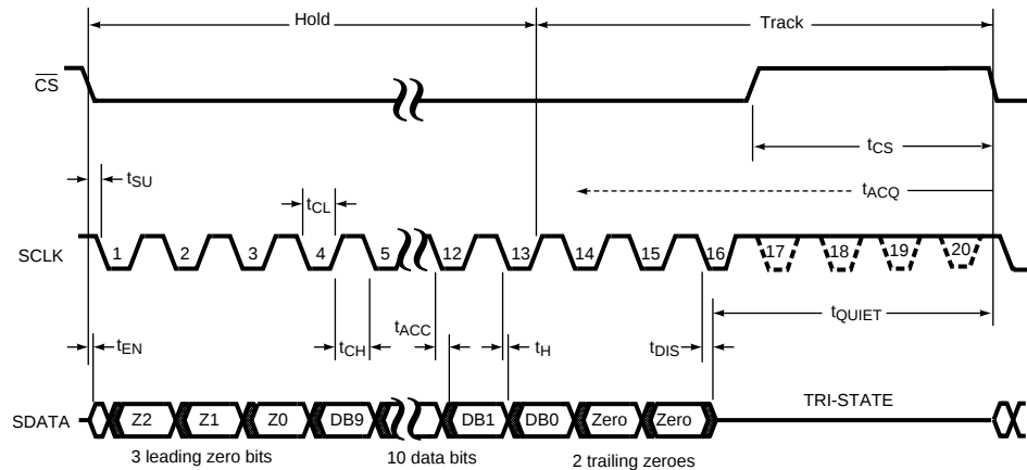
Figure 2. ADC101S051 Serial Timing Diagram
