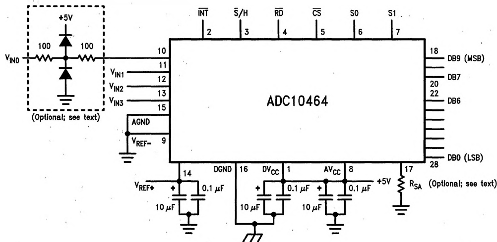
FIGURE 4. Typical Connection. Note the multiple bypass capacitors on the reference and power supply pins. If V_{REF} is not grounded, it should also be bypassed to analog ground using multiple capacitors (see 5.0 “Power Supply Considerations”). AGND and DGND should be at the same potential. V_{IN0} is shown with an input protection network. Pin 17 is normally left open, but optional “speedup” resistor R_{SA} can be used to reduce the conversion time.
