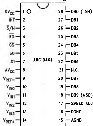
Dual-In-Line Package
