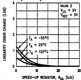
Linearity Change vs Speed-Up Resistor
