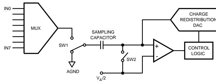
Figure 5. ADC108S052 in Hold Mode
