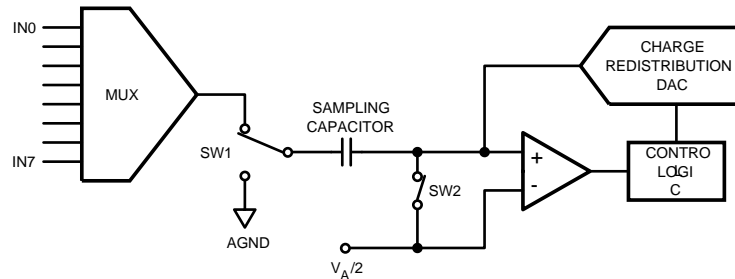
Figure 4. ADC108S052 in Track Mode
