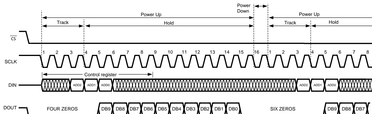
Figure 1. ADC108S052 Operational Timing Diagram
