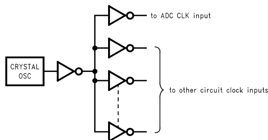
Figure 7. Isolating the ADC clock from Digital Circuitry.
