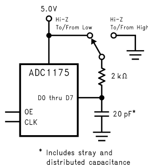
Figure 3. t_{EN} , t_{DIS} Test Circuit
