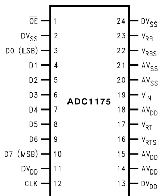
Figure 1. ADC1175 Pin Configuration
