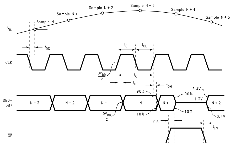
Figure 2. ADC1175 Timing Diagram
