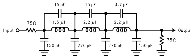
Figure 9. 11 MHz Low Pass Filter to Eliminate Harmonics at the Signal Input
