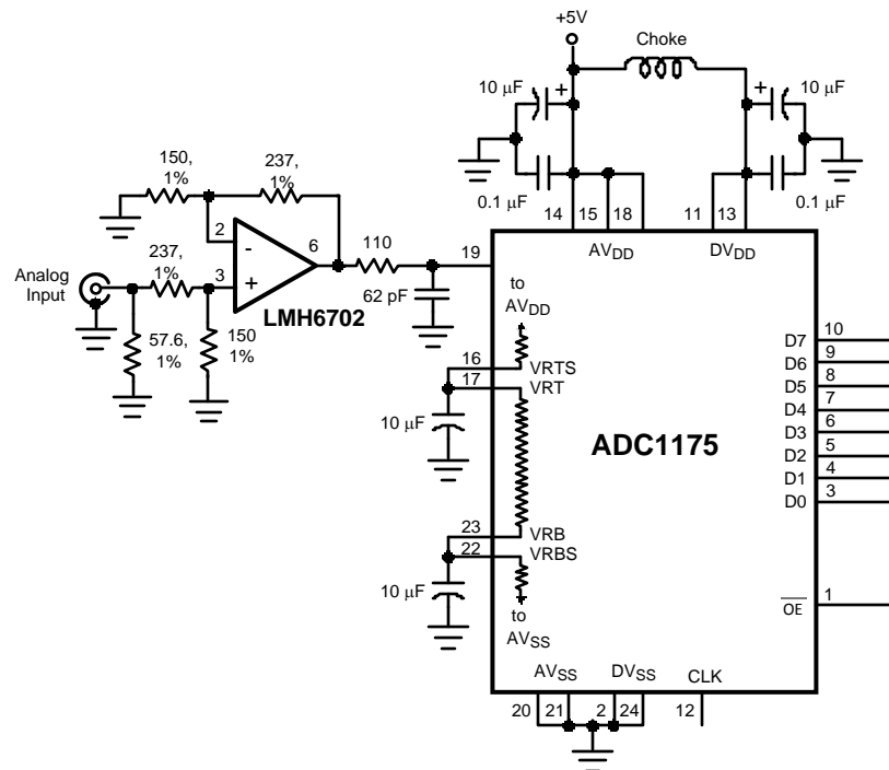
Figure 4. Simple, Low Component Count, Self-Bias Reference Application
