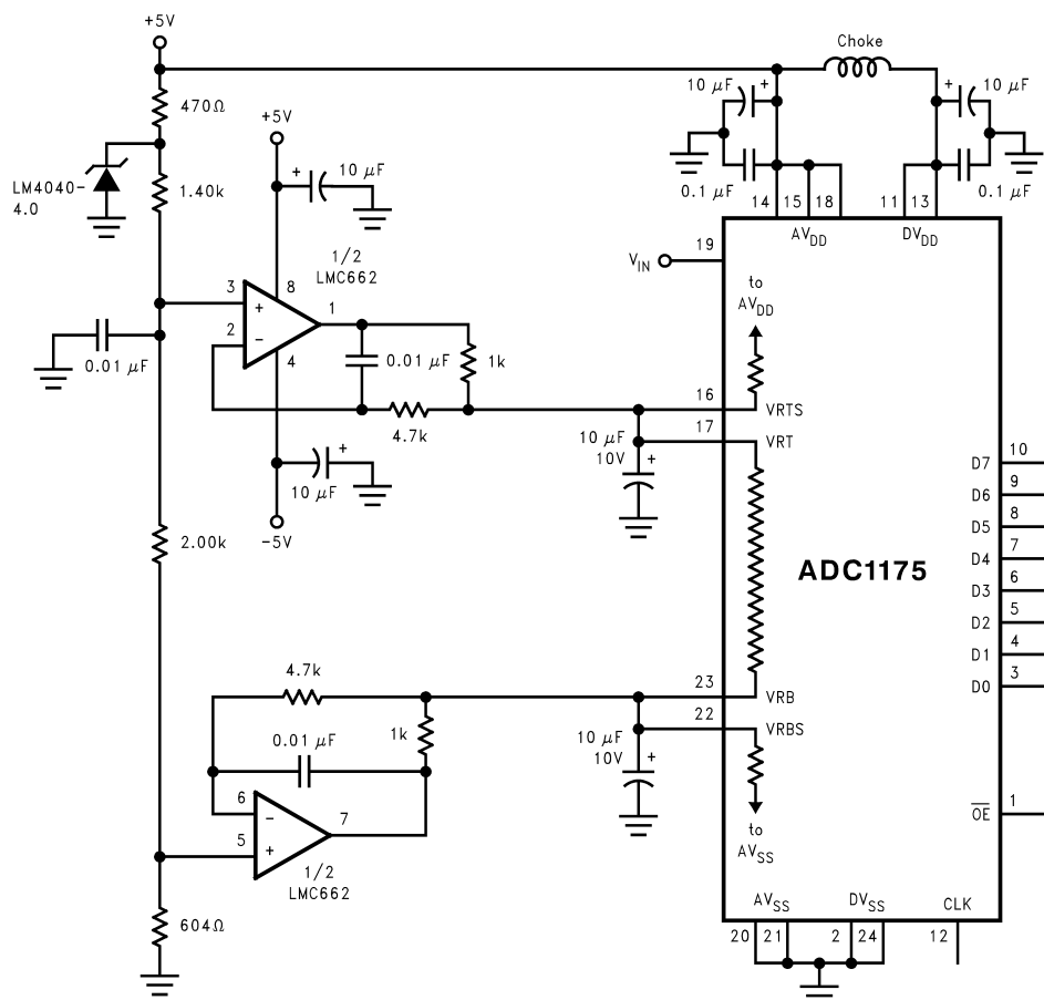
Figure 5. Better Defining the ADC Reference Voltage
