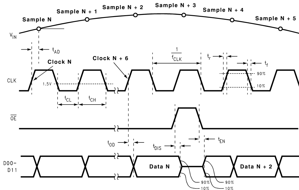
Output Timing
