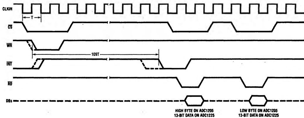
FIGURE 3. Timing Diagram
