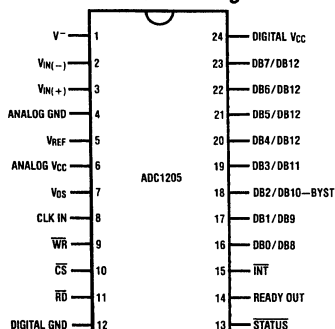
Dual-In-Line Package
