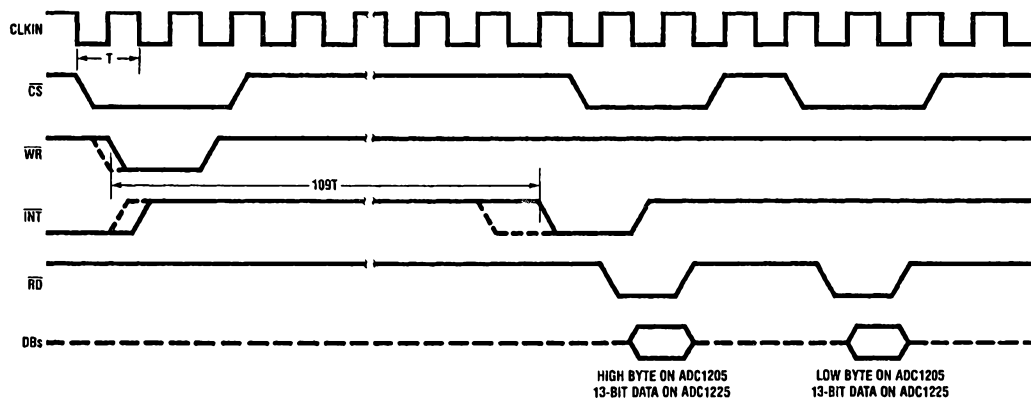
FIGURE 3. Timing Diagram
