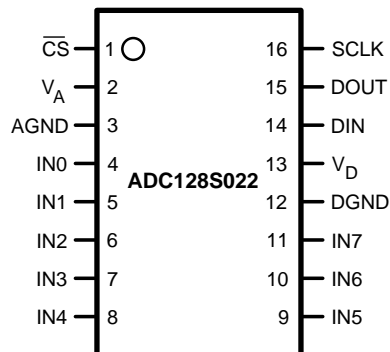
Figure 1. TSSOP
