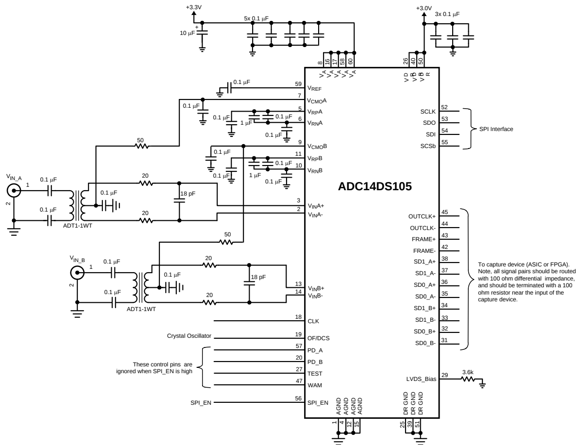
Figure 22. Application Circuit
