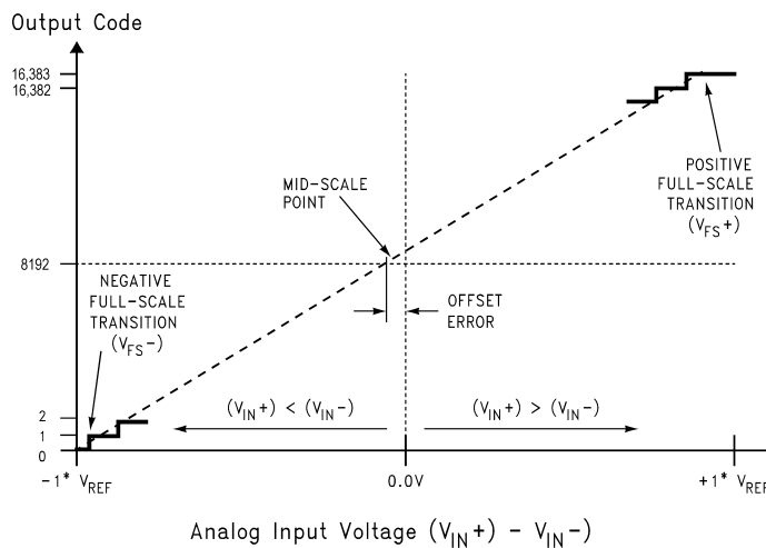
Figure 2. Transfer Characteristic
