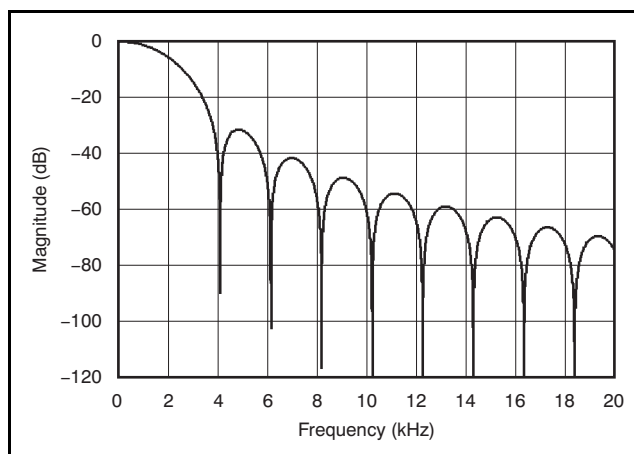
Figure 64. Filter Profile with Data Rate = 2kSPS
