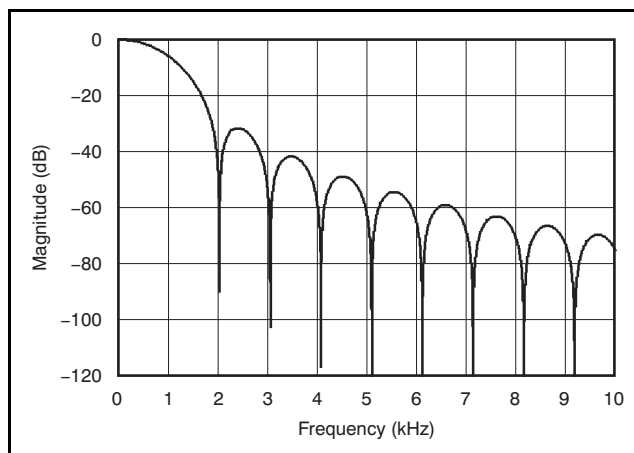
Figure 63. Filter Profile with Data Rate = 1kSPS
