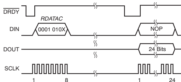
Figure 76. Read Data Continuously
