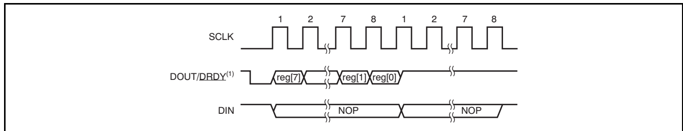
Figure 72. DOUT/DRDY Forced High After Reading Register Data
