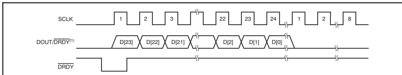
Figure 69. Data Retrieval with the \overline{\text{DRDY}} MODE Bit = 0 (Disabled)
