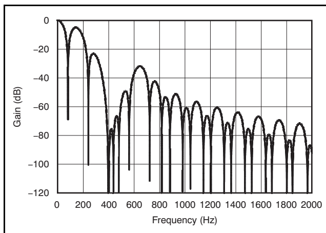
Figure 59. Filter Profile with Data Rate = 80SPS
