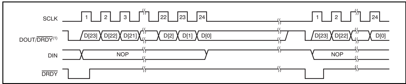
Figure 70. Data Retrieval with the DRDY MODE Bit = 1 (Enabled)
