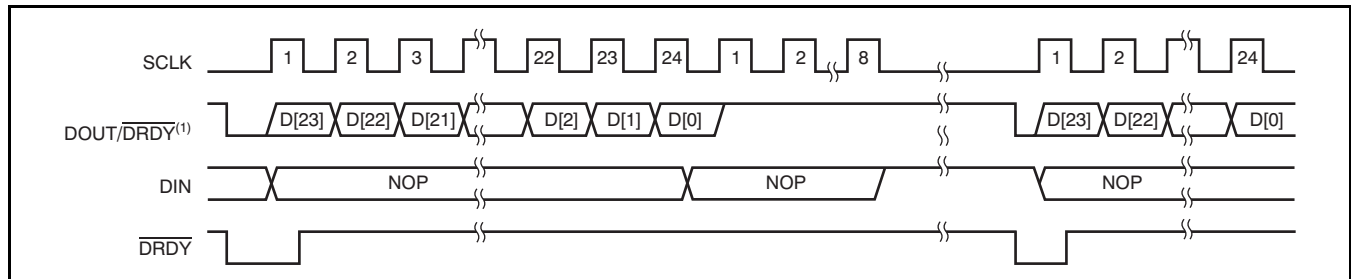
Figure 71. DOUT/DRDY Forced High After Retrieving the Conversion Result
