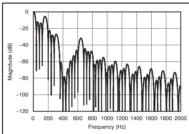
Figure 58. Filter Profile with Data Rate = 40SPS
