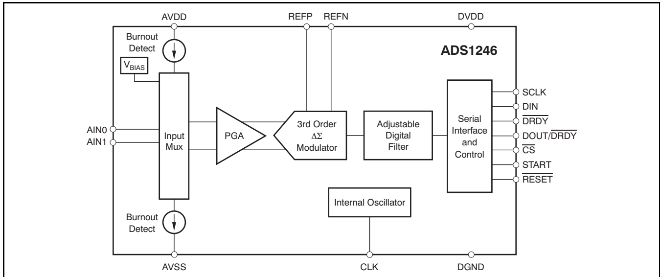
Figure 49. ADS1246 Diagram
