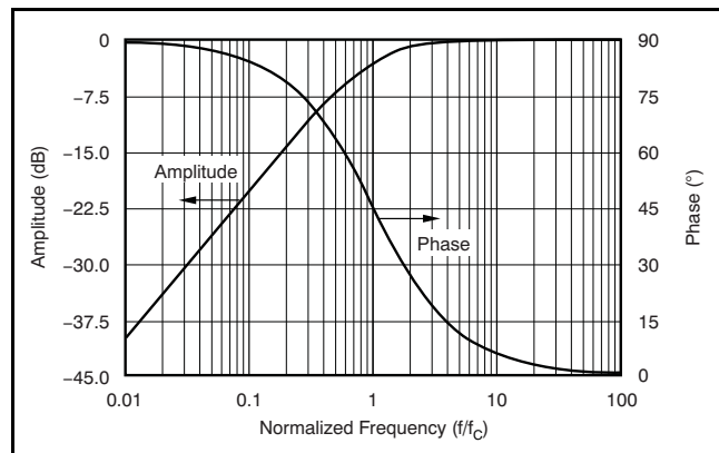
Figure 52. HPF Amplitude and Phase Response
