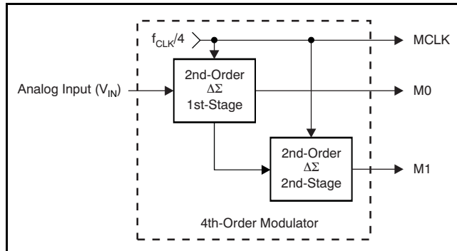
Figure 37. Fourth-Order Modulator
