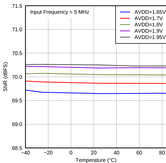
Figure 23. Signal-to-Noise Ratio Across AVDD and Temperature
