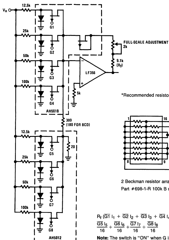
8-Bit Binary (BCD) Multiplying D/A Converter*
