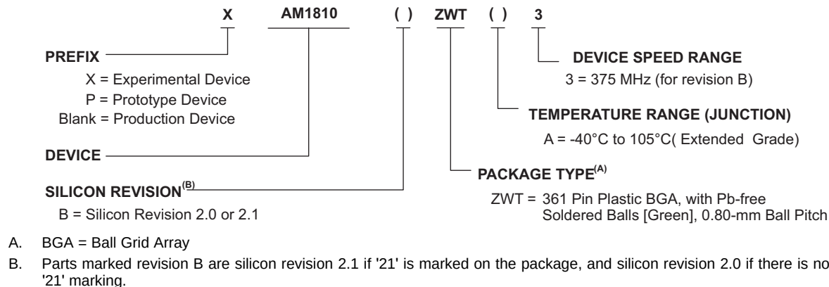
Figure 6-1. Device Nomenclature
