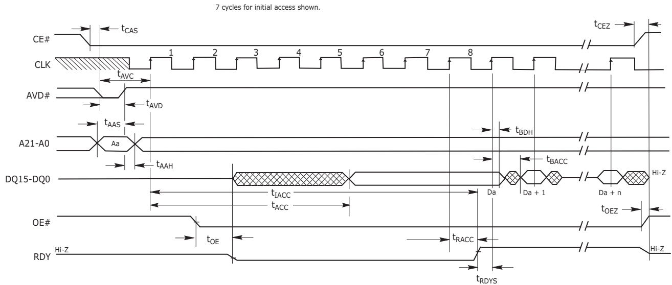
Figure I7. Reduced Wait-State Handshaking Burst Mode Read Starting at an Odd Address
