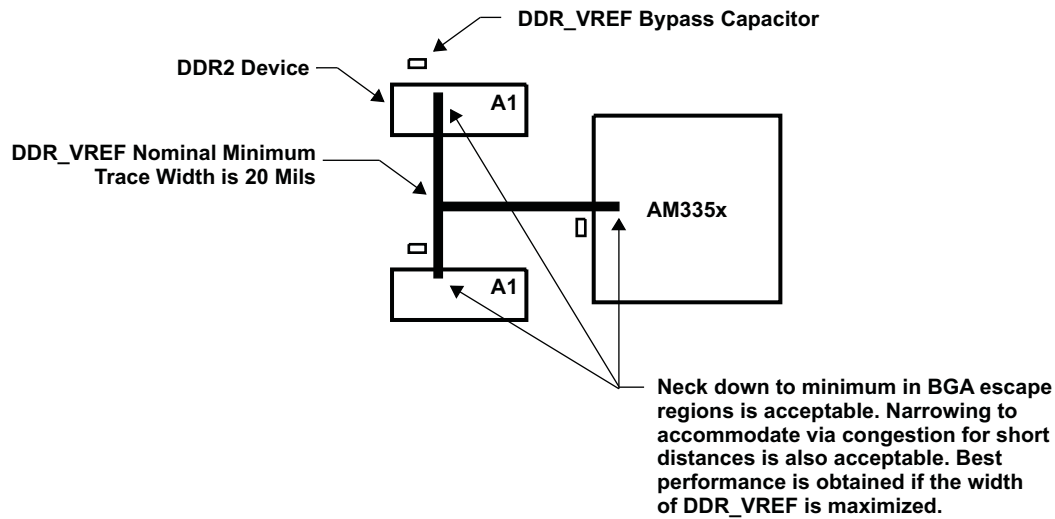
Figure 5-42. DDR_VREF Routing and Topology
