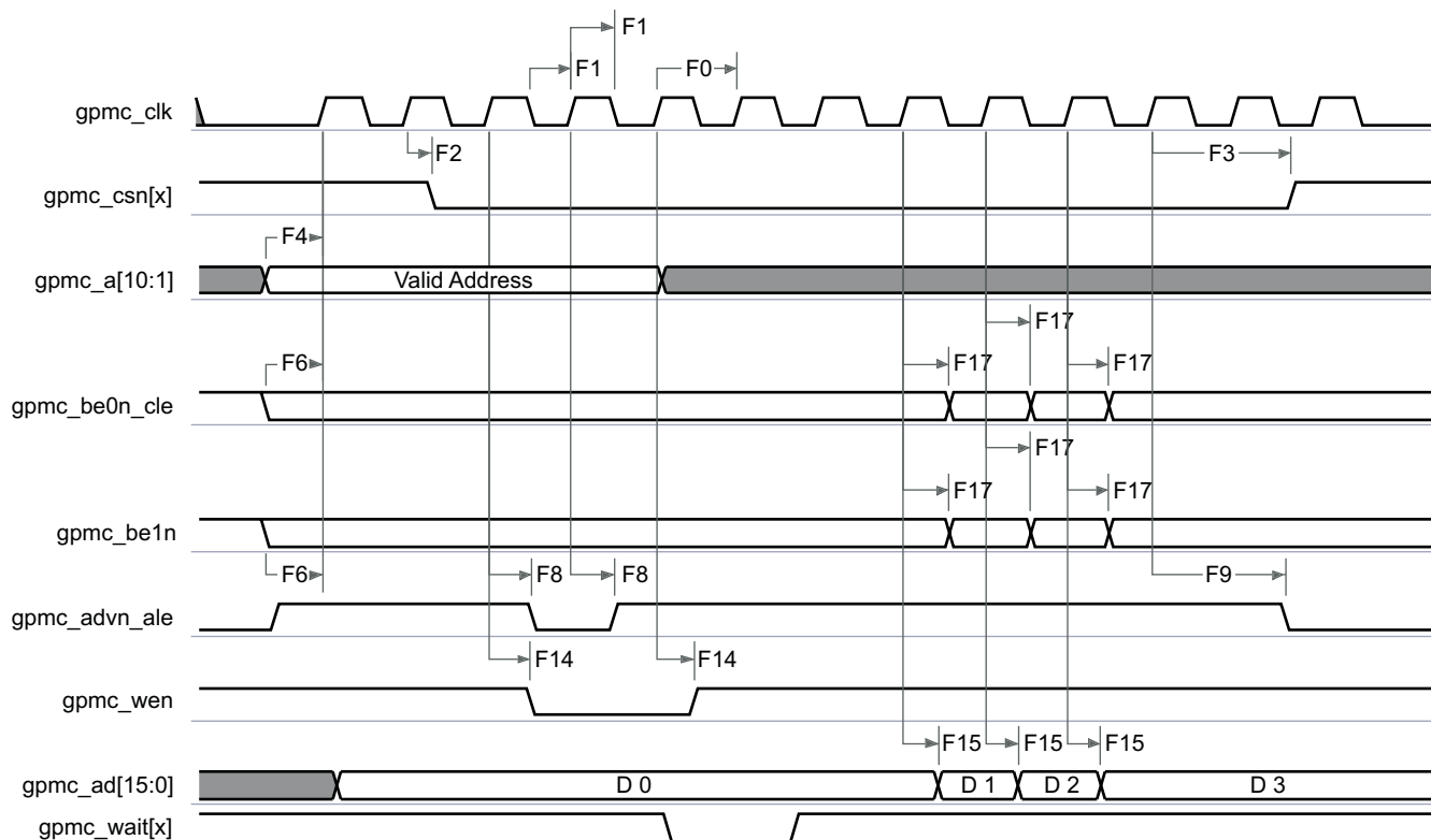
Figure 5-18. GPMC and NOR Flash—Synchronous Burst Write—(GpmcFCLKDivider > 0)
