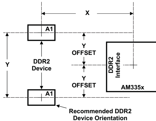
Figure 5-40. AM335x Device and DDR2 Device Placement
