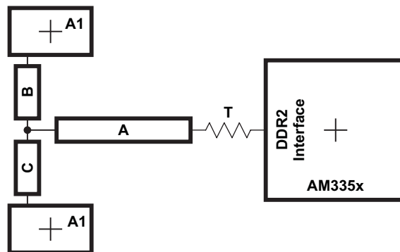
Figure 5-43. CK and ADDR_CTRL Routing and Topology
