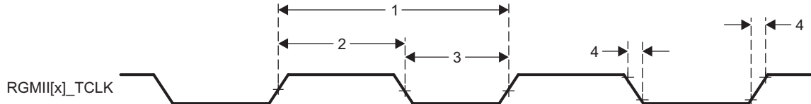
Figure 5-14. RGMII[x]_TCLK Timing - RGMII Mode
