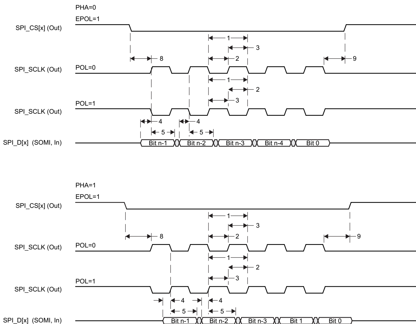
Figure 5-88. SPI Master Mode Receive Timing
