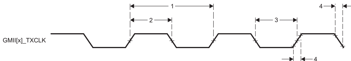
Figure 5-6. GMII[x]_TXCLK Timing - MII Mode
