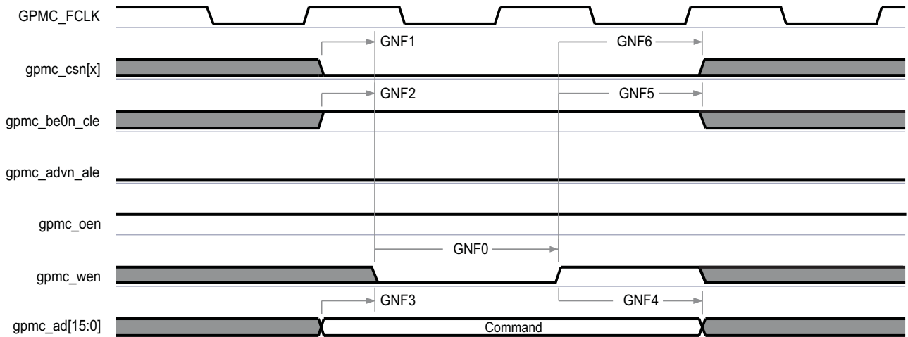
Figure 5-27. GPMC and NAND Flash—Command Latch Cycle
