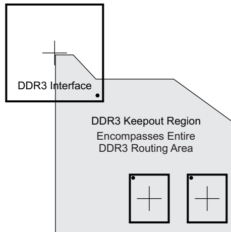
Figure 5-50. DDR3 Keepout Region
