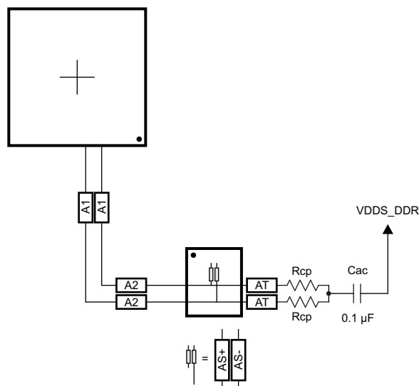
Figure 5-59. CK Routing for One DDR3 Device
