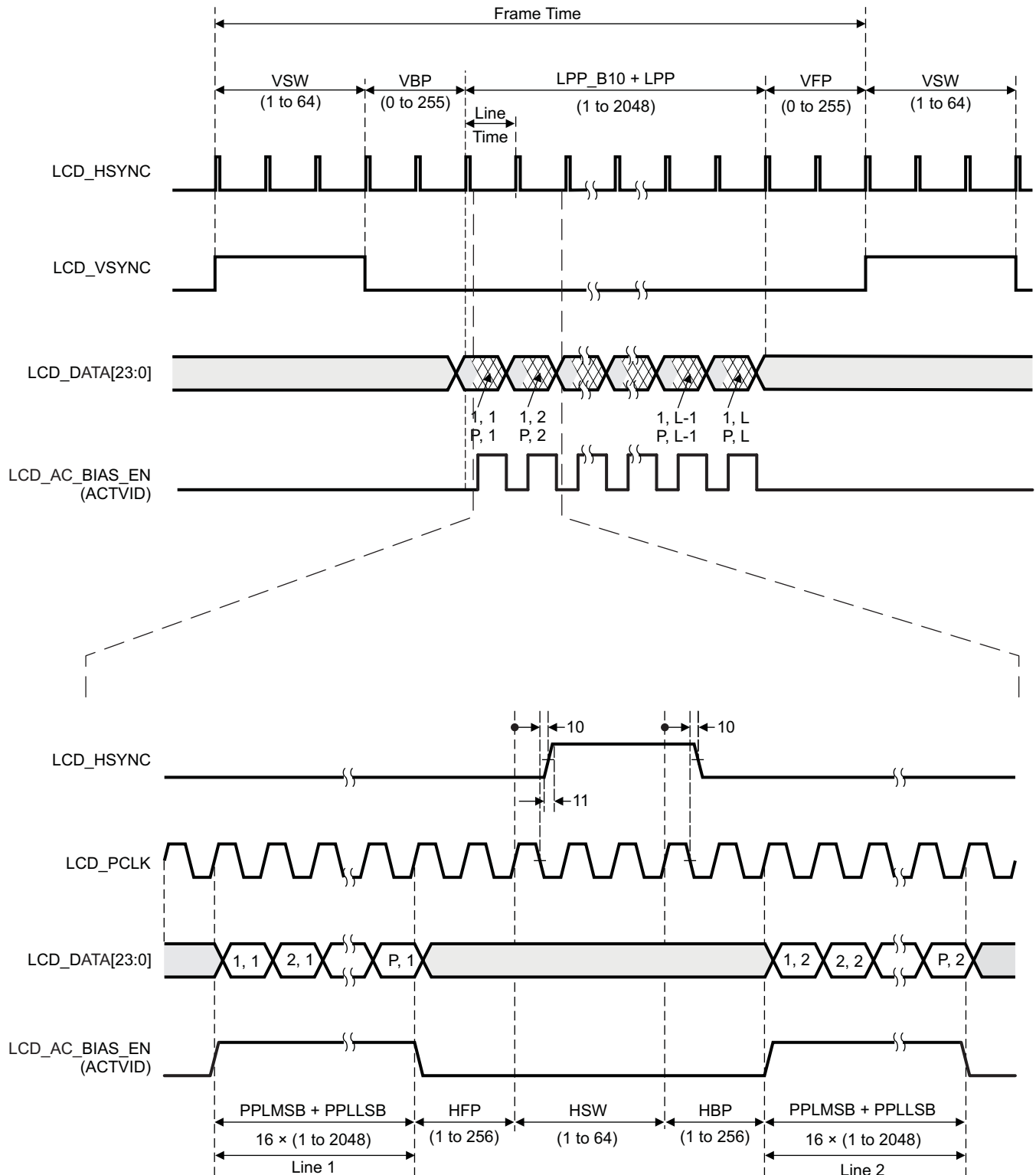
Figure 5-80. LCD Raster-Mode Active
