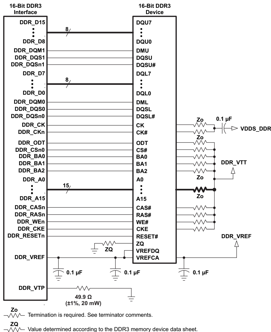
Figure 5-46. 16-Bit DDR3 Interface Using One 16-Bit DDR3 Device with V_{TT} Termination
