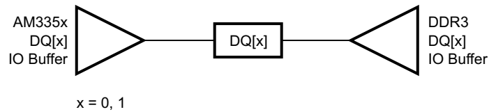
Figure 5-62. DQ[x] Topology
