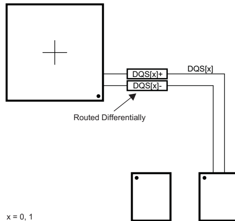
Figure 5-63. DQS[x] Routing With Any Number of Allowed DDR3 Devices
