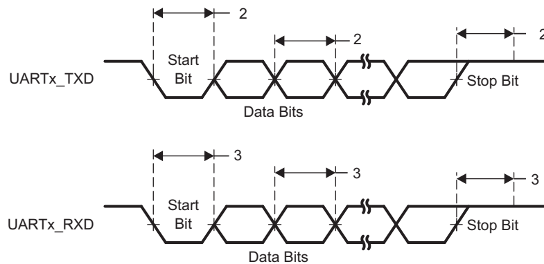
Figure 5-94. UART Timings
