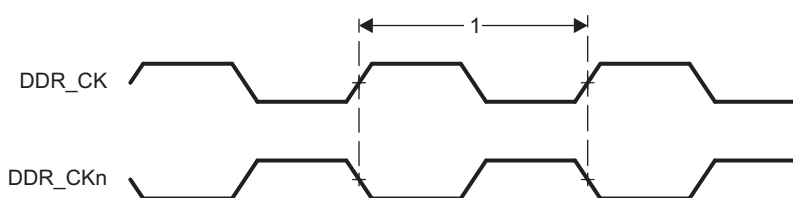
Figure 5-37. DDR2 Memory Interface Clock Timing
