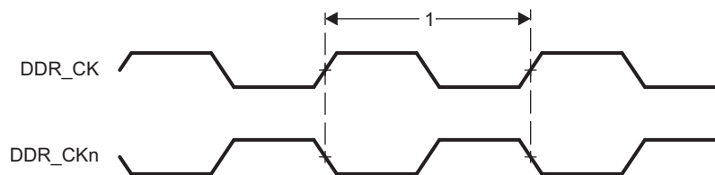
Figure 5-31. LPDDR Memory Interface Clock Timing
