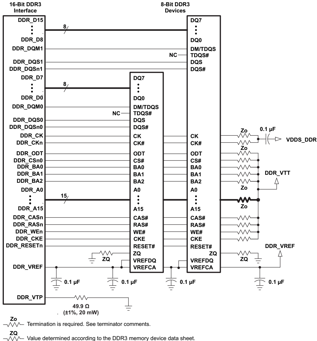
Figure 5-48. 16-Bit DDR3 Interface Using Two 8-Bit DDR3 Devices
