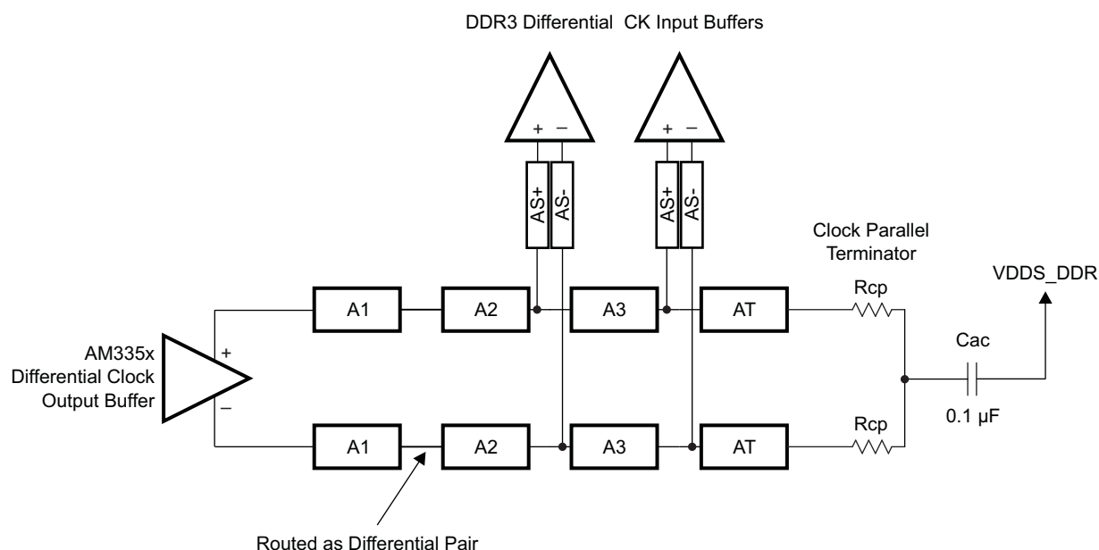
Figure 5-51. CK Topology for Two DDR3 Devices
