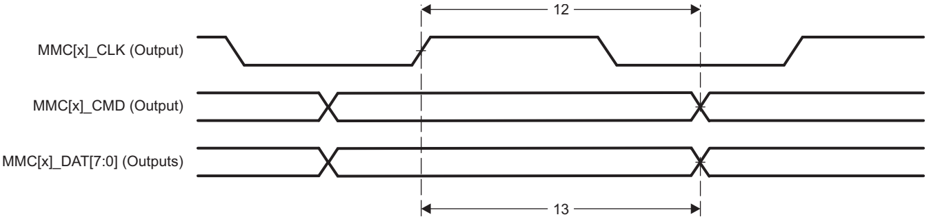
Figure 5-93. MMC[x]_CMD and MMC[x]_DAT[7:0] Output Timing—High Speed Mode
