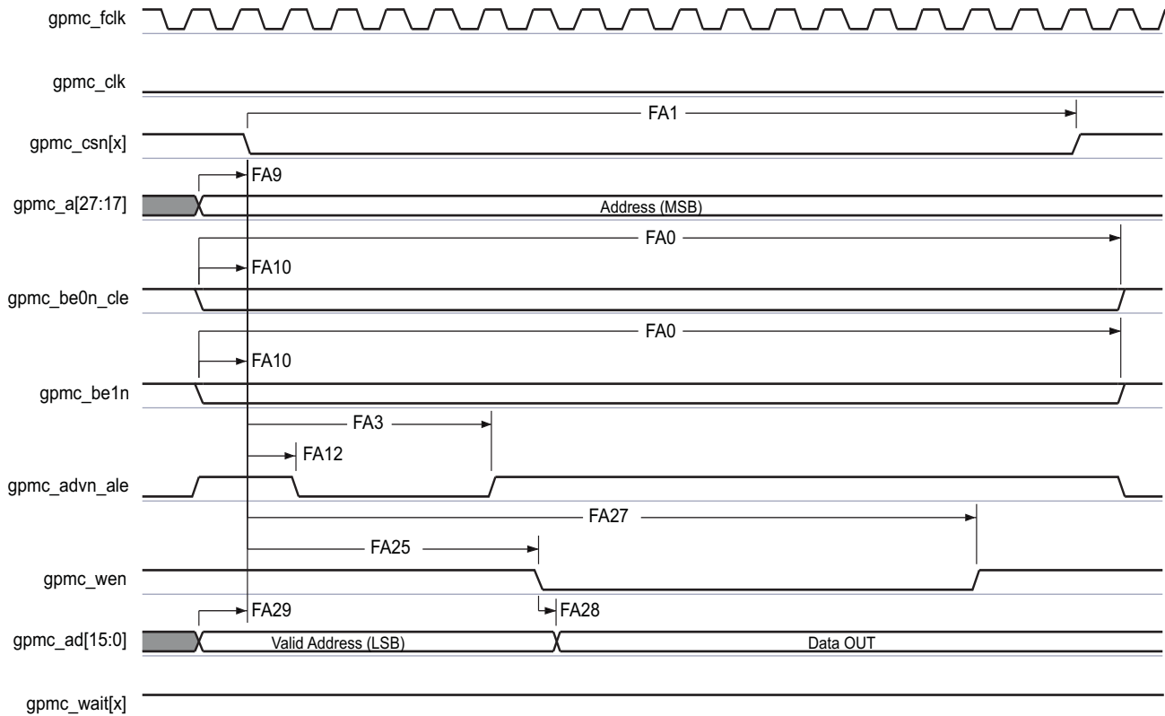
Figure 5-26. GPMC and Multiplexed NOR Flash—Asynchronous Write—Single Word
