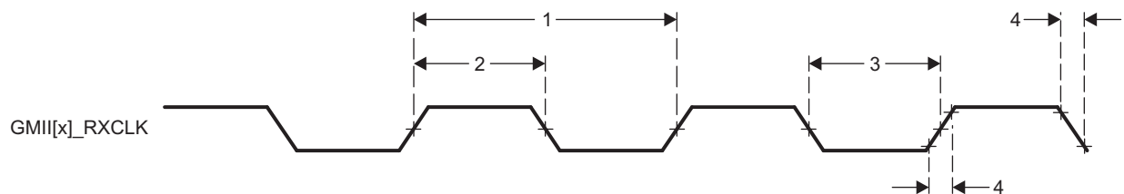
Figure 5-5. GMII[x]_RXCLK Timing - MII Mode
