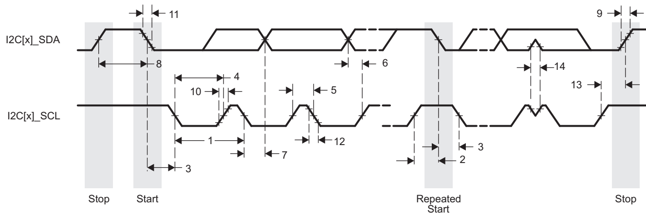
Figure 5-67. I2C Receive Timing
