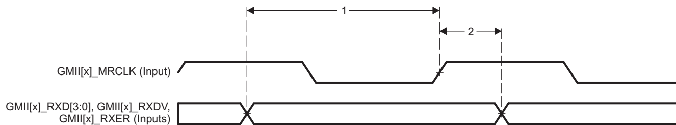
Figure 5-7. GMII[x]_RXD[3:0], GMII[x]_RXDV, GMII[x]_RXER Timing - MII Mode
