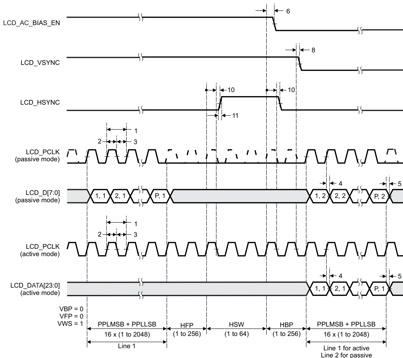
Figure 5-83. LCD Raster-Mode Control Signal Deactivation
