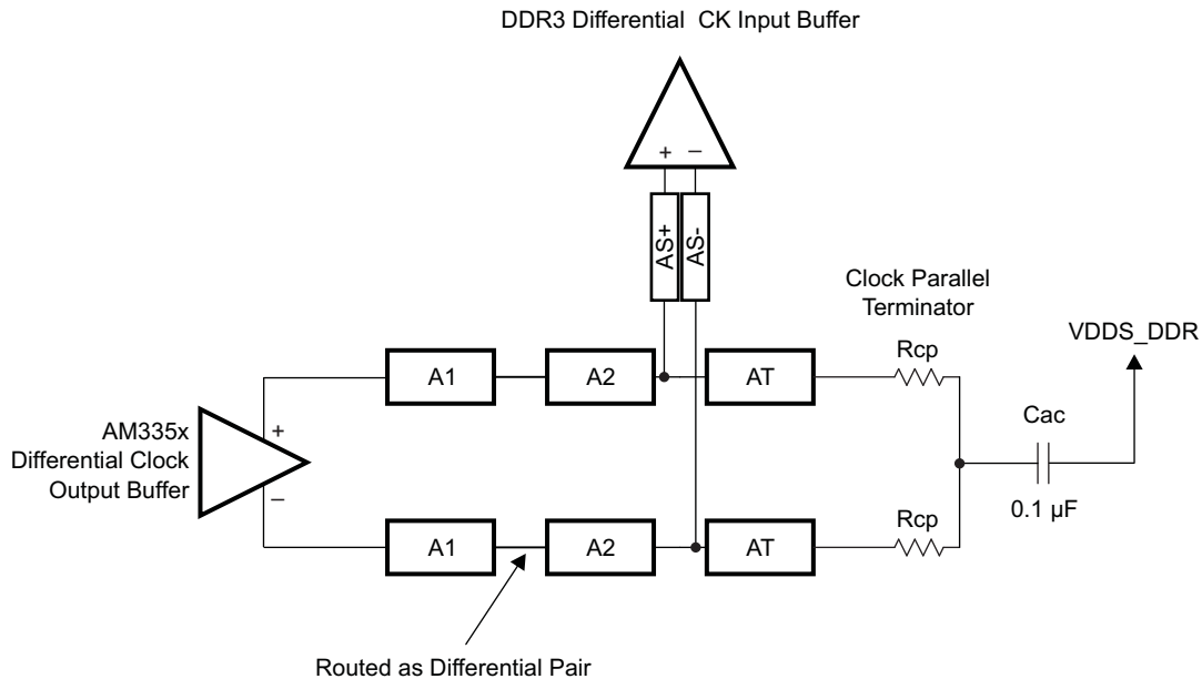
Figure 5-57. CK Topology for One DDR3 Device
