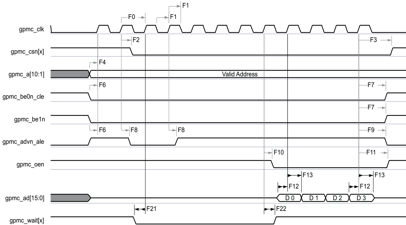
Figure 5-17. GPMC and NOR Flash—Synchronous Burst Read—4x16-bit (GpmcFCLKDivider = 0)
