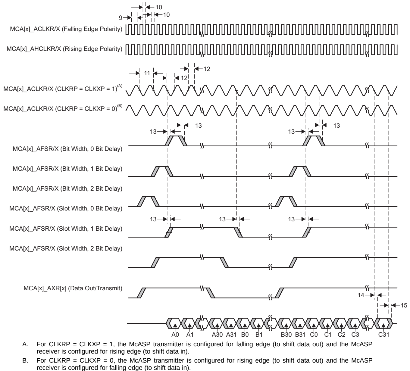
Figure 5-85. McASP Output Timing
