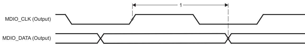
Figure 5-4. MDIO_DATA Timing - Output Mode
