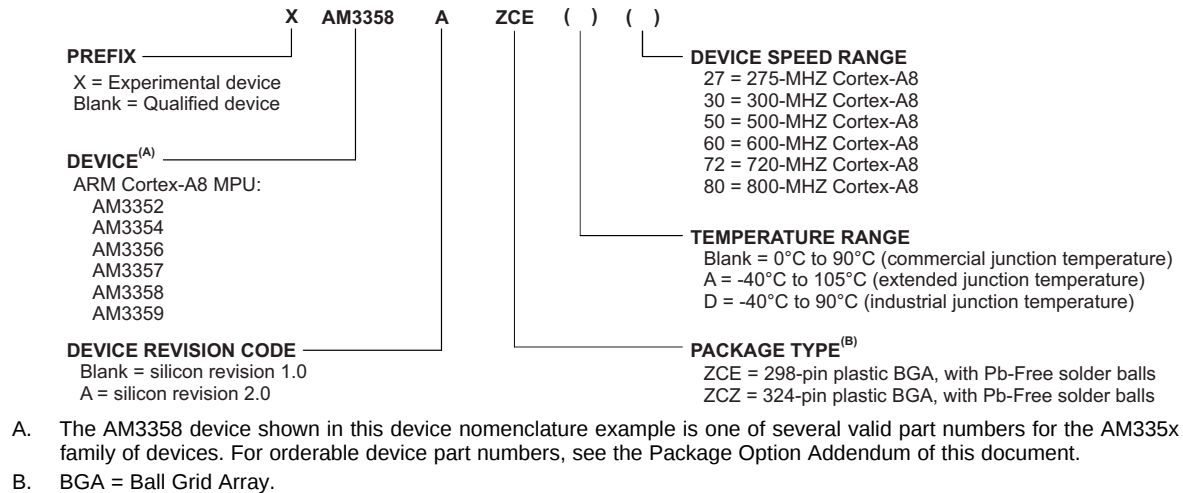
Figure 6-1. AM335x Device Nomenclature
