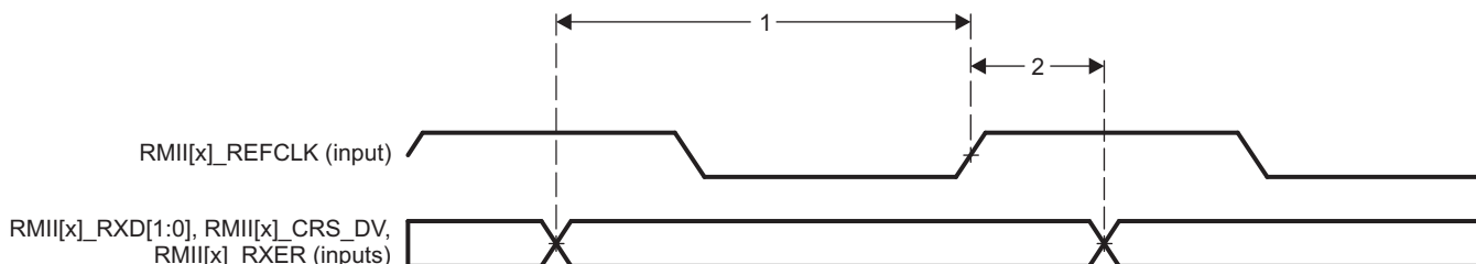
Figure 5-10. RMII[x]_RXD[1:0], RMII[x]_CRS_DV, RMII[x]_RXER Timing - RMII Mode
