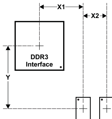
Figure 5-49. Placement Specifications
