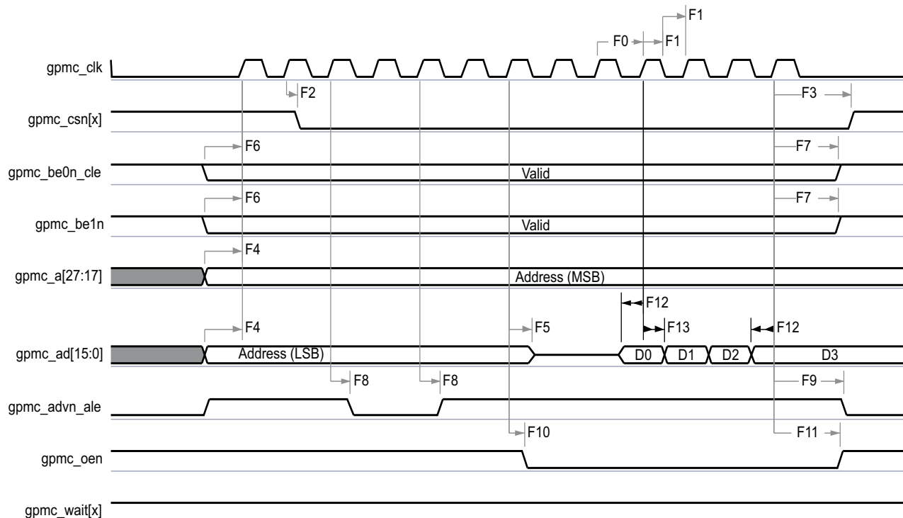
Figure 5-19. GPMC and Multiplexed NOR Flash—Synchronous Burst Read
