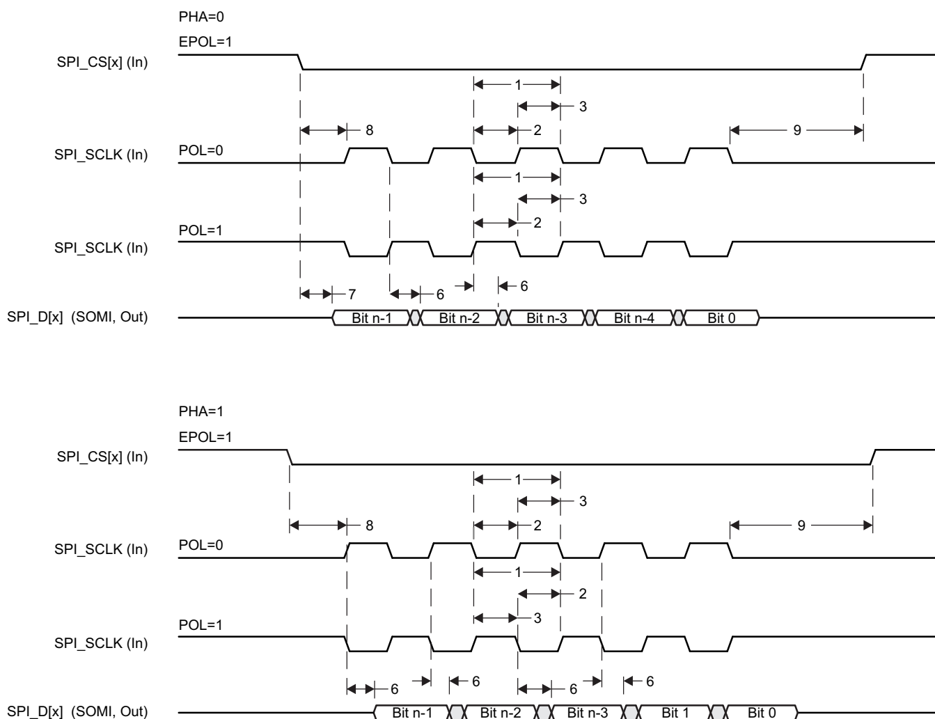
Figure 5-87. SPI Slave Mode Transmit Timing
