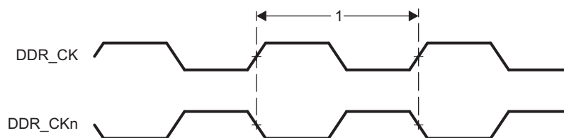
Figure 5-45. DDR3 Memory Interface Clock Timing
