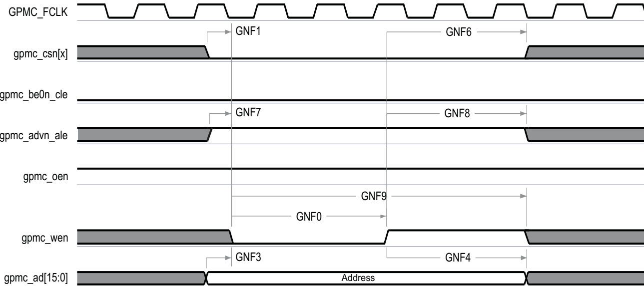
Figure 5-28. GPMC and NAND Flash—Address Latch Cycle
