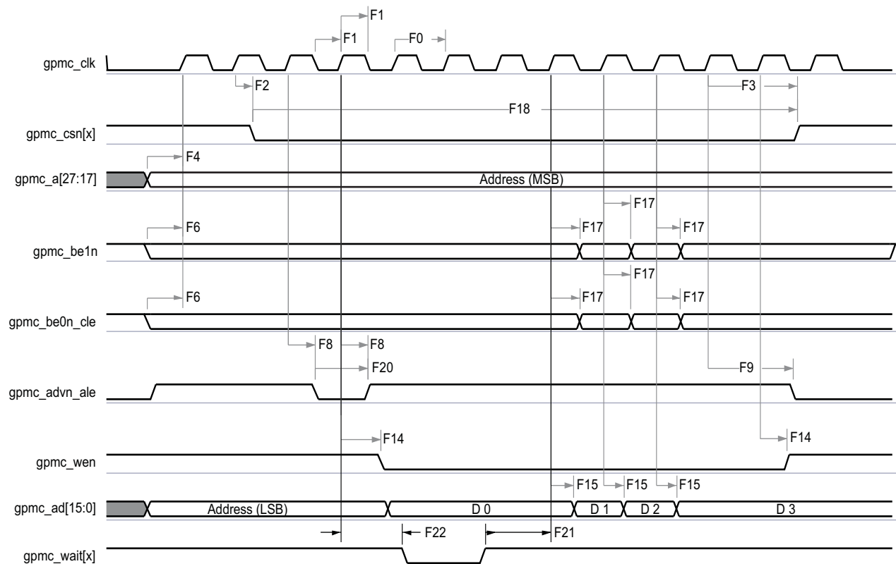
Figure 5-20. GPMC and Multiplexed NOR Flash—Synchronous Burst Write
