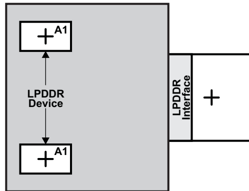
Figure 5-34. LPDDR Keepout Region
