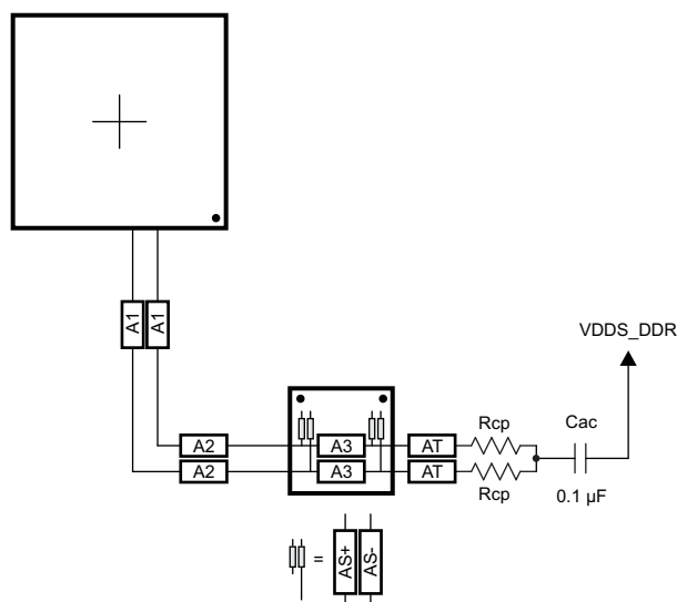
Figure 5-55. CK Routing for Two Mirrored DDR3 Devices
