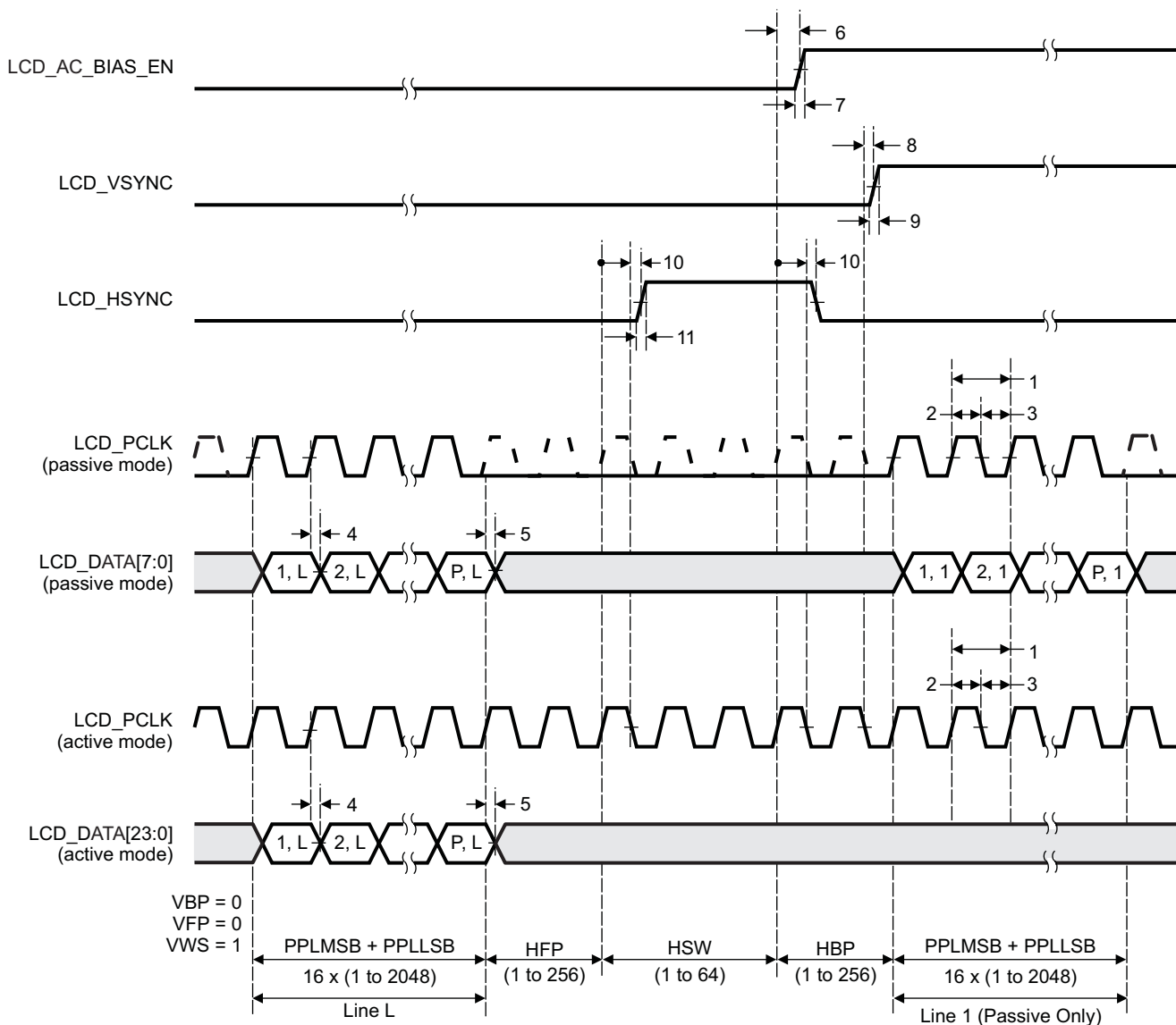
Figure 5-82. LCD Raster-Mode Control Signal Activation
