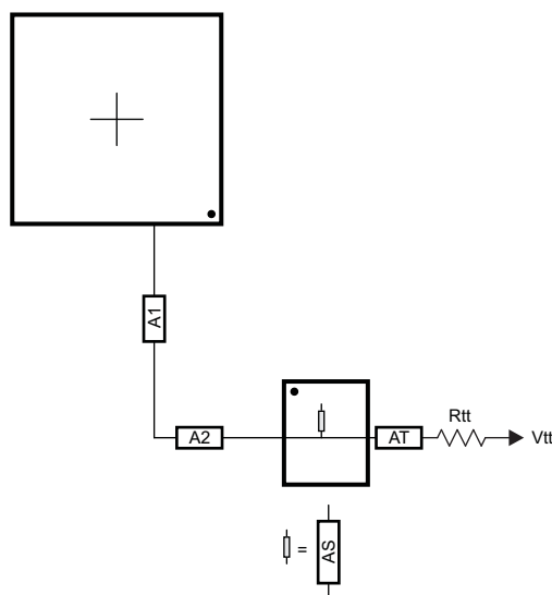
Figure 5-60. ADDR_CTRL Routing for One DDR3 Device
