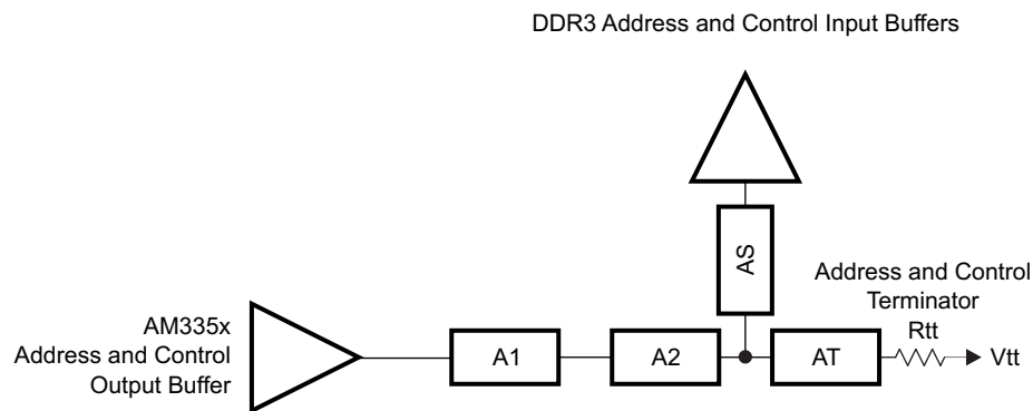
Figure 5-58. ADDR_CTRL Topology for One DDR3 Device
