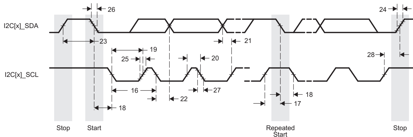
Figure 5-68. I2C Transmit Timing
