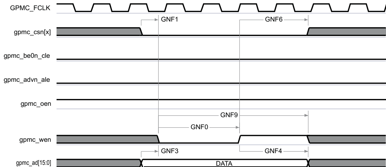
Figure 5-30. GPMC and NAND Flash—Data Write Cycle
