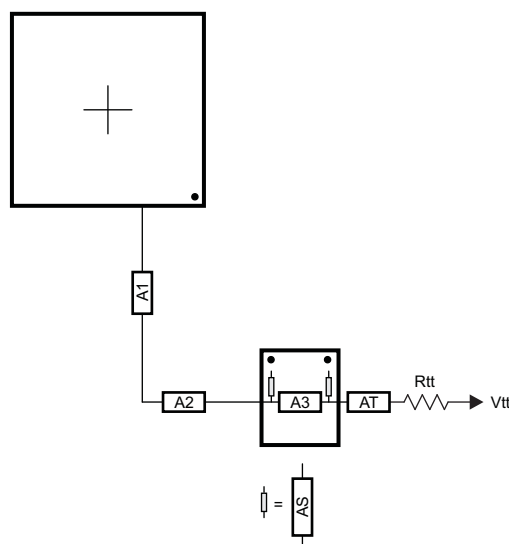
Figure 5-56. ADDR_CTRL Routing for Two Mirrored DDR3 Devices
