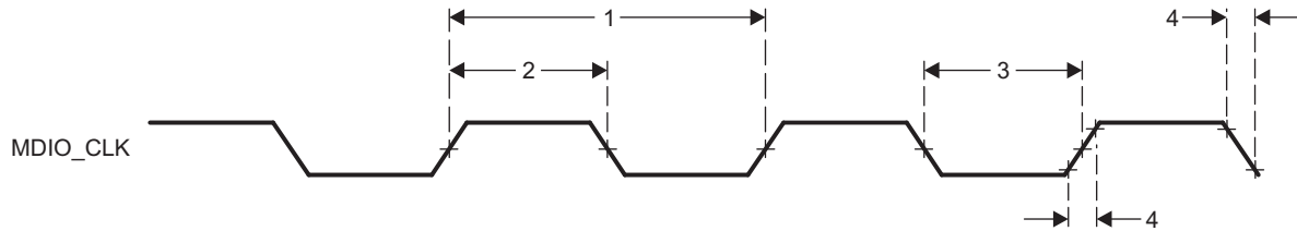
Figure 5-3. MDIO_CLK Timing
