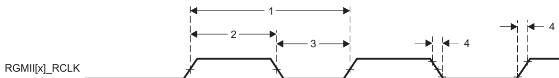
Figure 5-12. RGMII[x]_RCLK Timing - RGMII Mode
