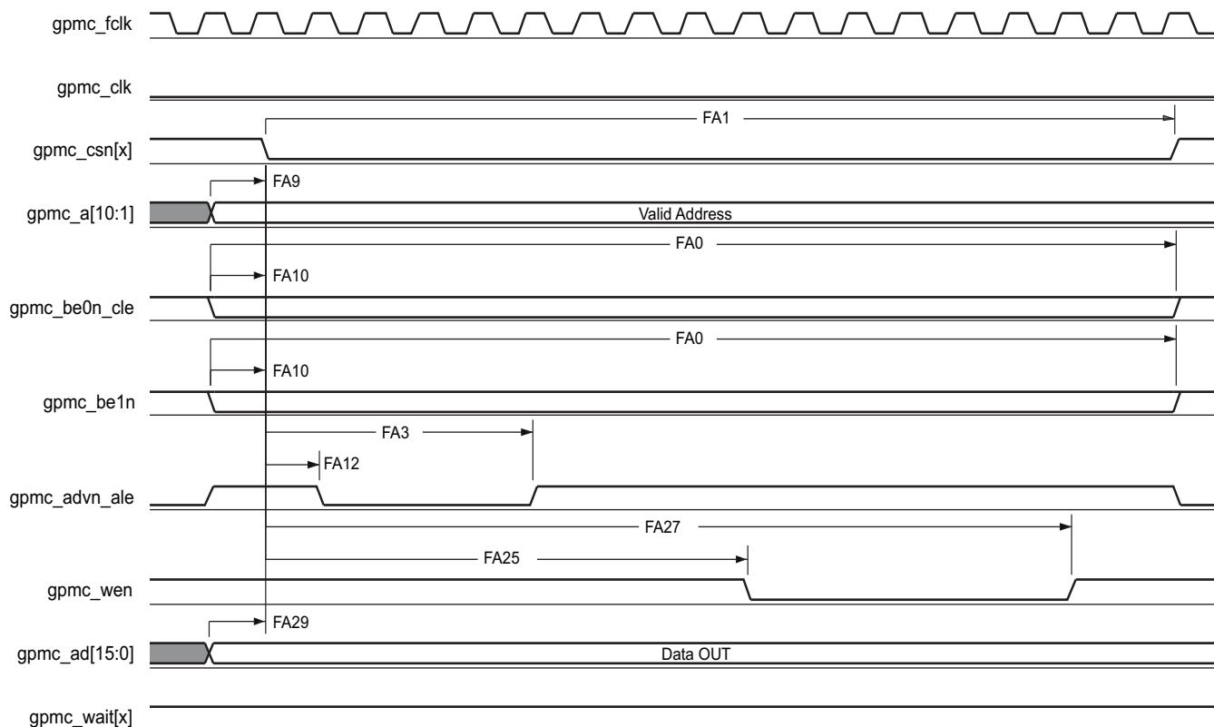
Figure 5-24. GPMC and NOR Flash—Asynchronous Write—Single Word
