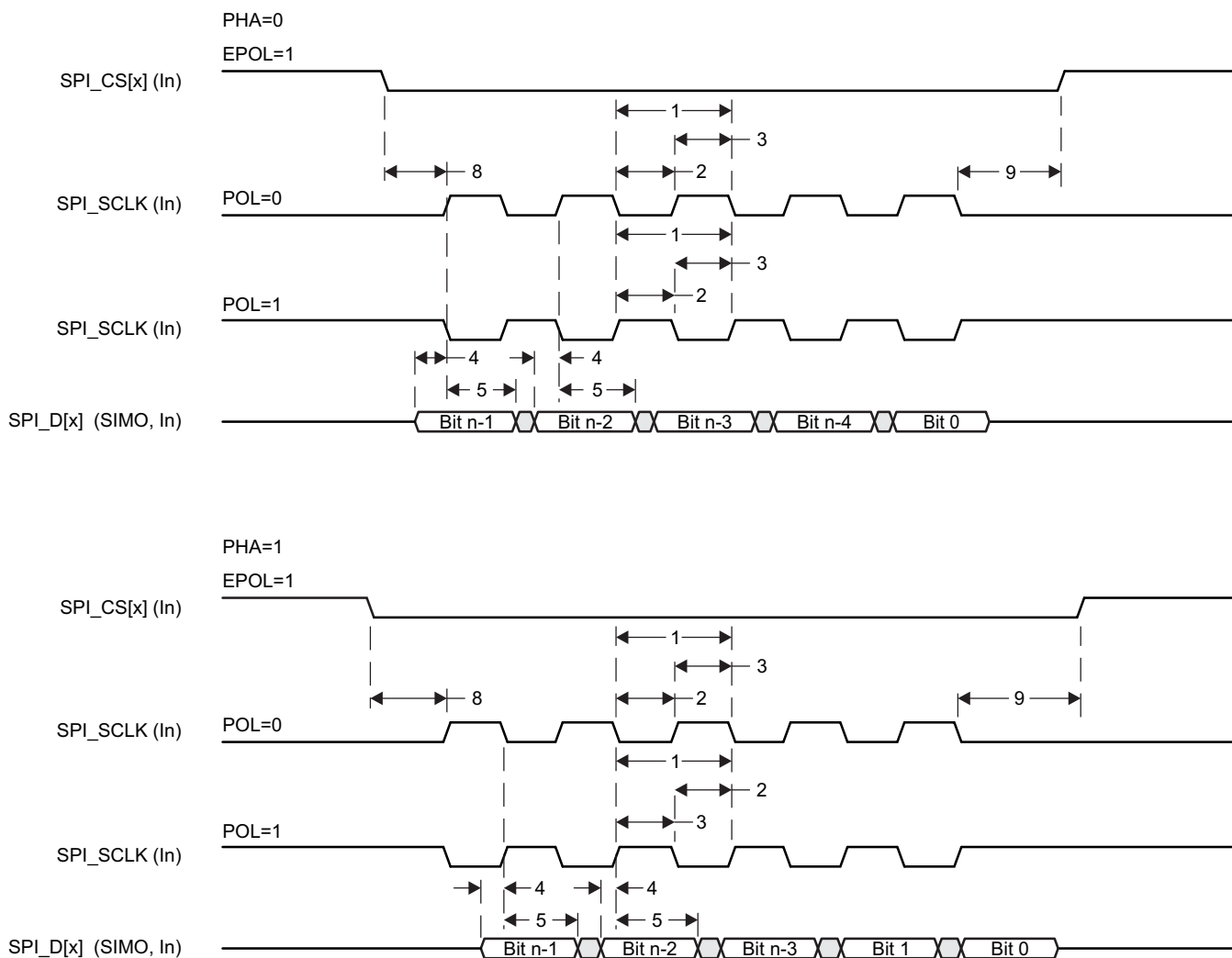
Figure 5-86. SPI Slave Mode Receive Timing
