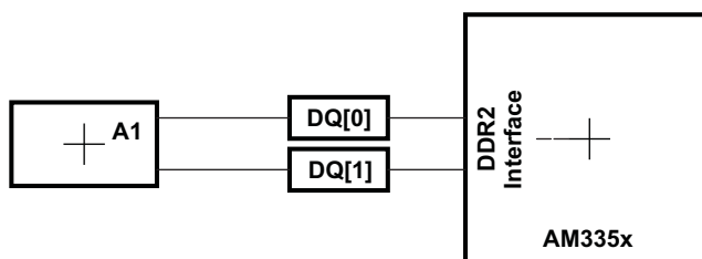
Figure 5-44. DQS[x] and DQ[x] Routing and Topology
