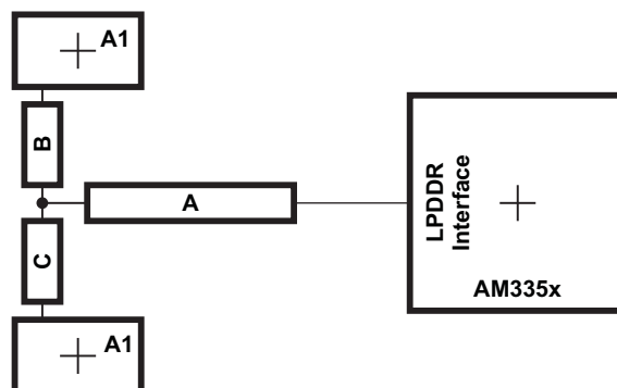
Figure 5-35. CK and ADDR_CTRL Routing and Topology
