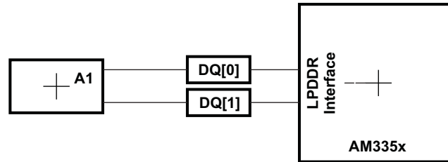
Figure 5-36. DQS[x] and DQ[x] Routing and Topology
