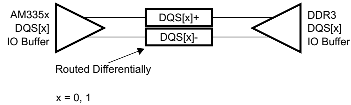
Figure 5-61. DQS[x] Topology
