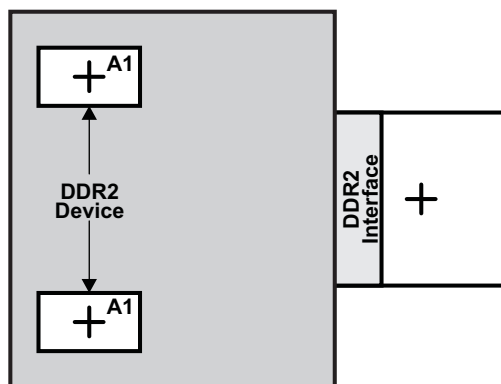
Figure 5-41. DDR2 Keepout Region
