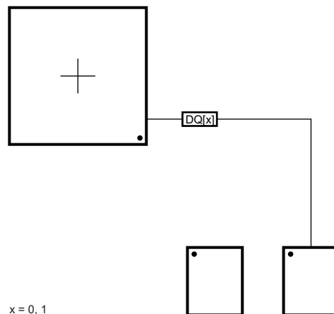
Figure 5-64. DQ[x] Routing With Any Number of Allowed DDR3 Devices
