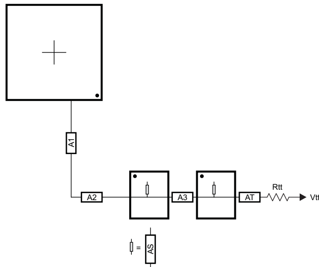
Figure 5-54. ADDR_CTRL Routing for Two Single-Side DDR3 Devices
