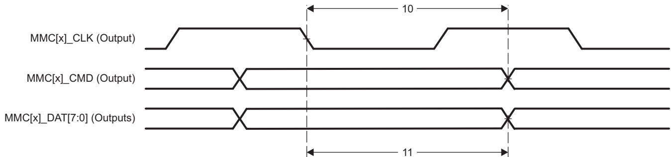
Figure 5-92. MMC[x]_CMD and MMC[x]_DAT[7:0] Output Timing—Standard Mode
