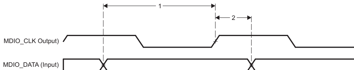
Figure 5-2. MDIO_DATA Timing - Input Mode
