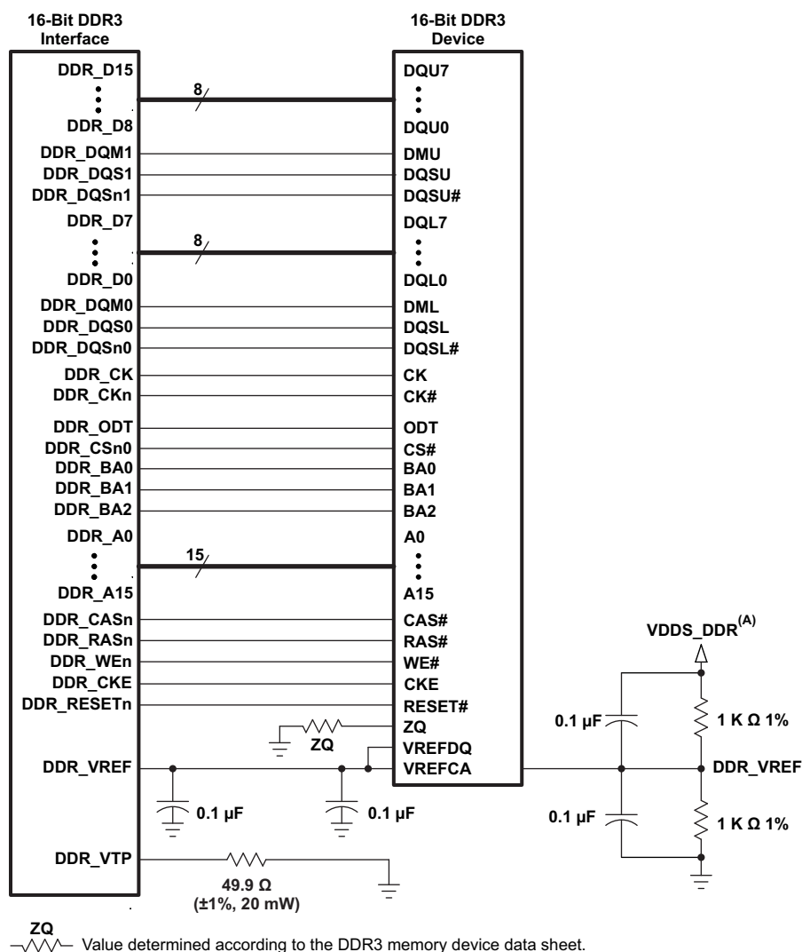
Figure 5-47. 16-Bit DDR3 Interface Using One 16-Bit DDR3 Device without V TT Termination
