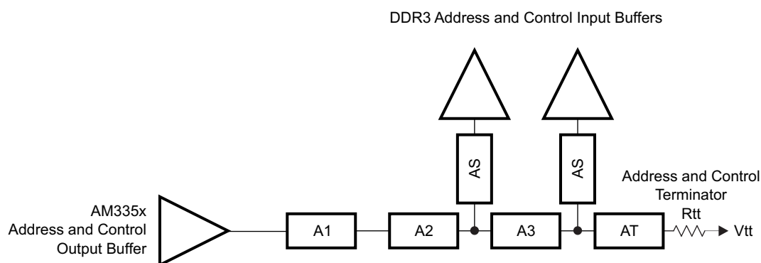
Figure 5-52. ADDR_CTRL Topology for Two DDR3 Devices
