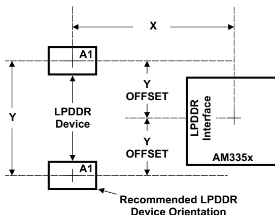
Figure 5-33. AM335x Device and LPDDR Device Placement
