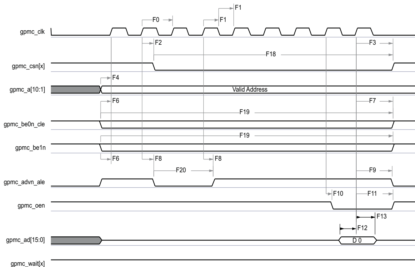
Figure 5-16. GPMC and NOR Flash—Synchronous Single Read—(GpmcFCLKDivider = 0)
