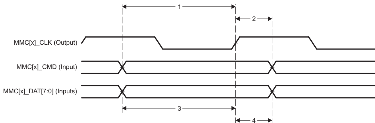
Figure 5-90. MMC[x]_CMD and MMC[x]_DAT[7:0] Input Timing
