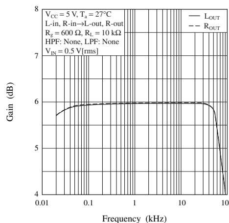
Gain — Frequency
