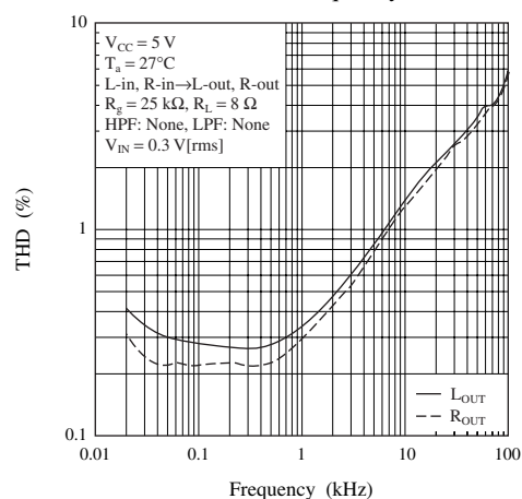
THD — Frequency
