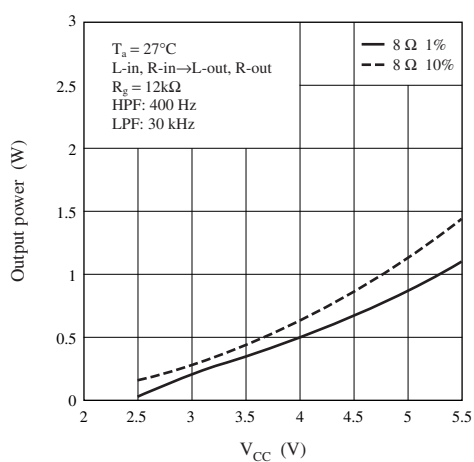
L-ch. 8 \Omega
