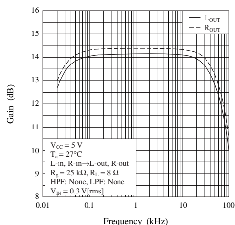
Gain — Frequency
