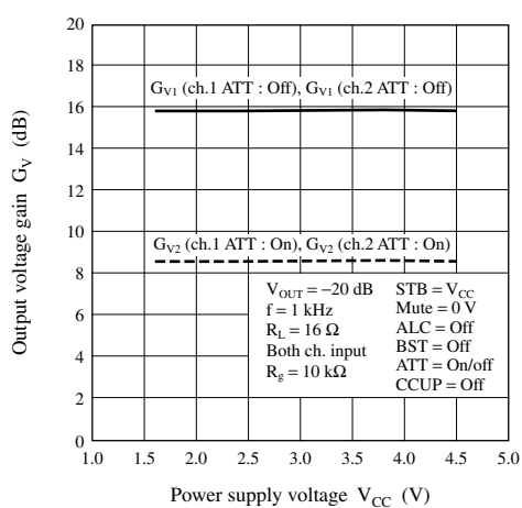
G_V - V_{CC}
