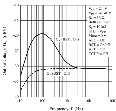
G_V — frequency
