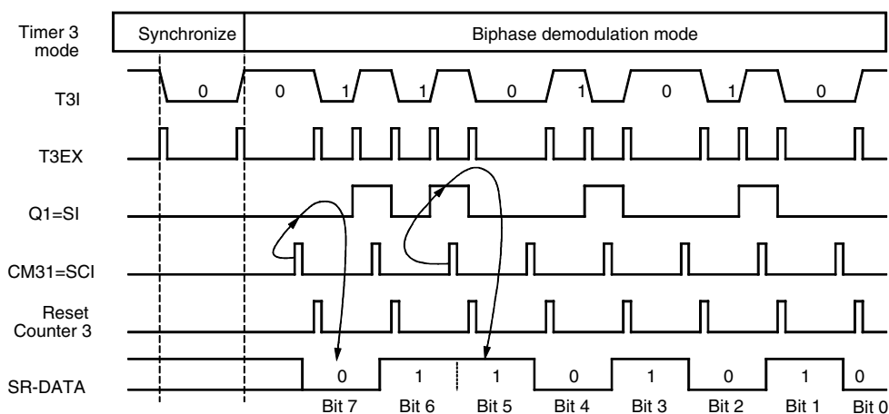
Figure 77. Bi-phase Demodulation
