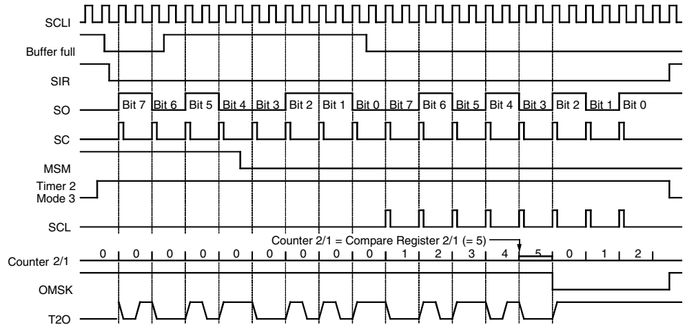
Figure 72. Bi-phase Modulation 2
