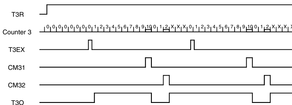
Figure 48. Externally Triggered Counter Reset and Start Combined with Single-action Mode
