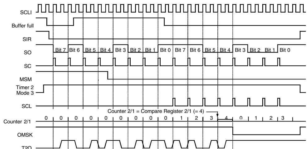
Figure 71. Manchester Modulation 2
