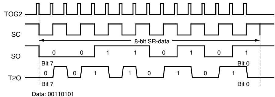
Figure 70. Manchester Modulation 1
