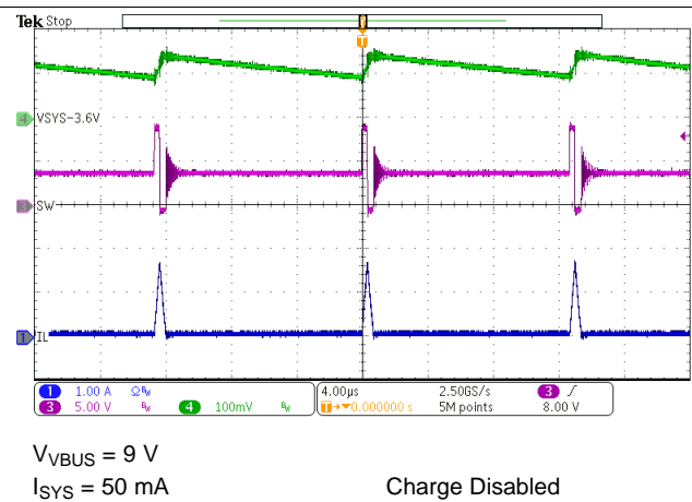
Figure 44. PFM Switching in Buck Mode
