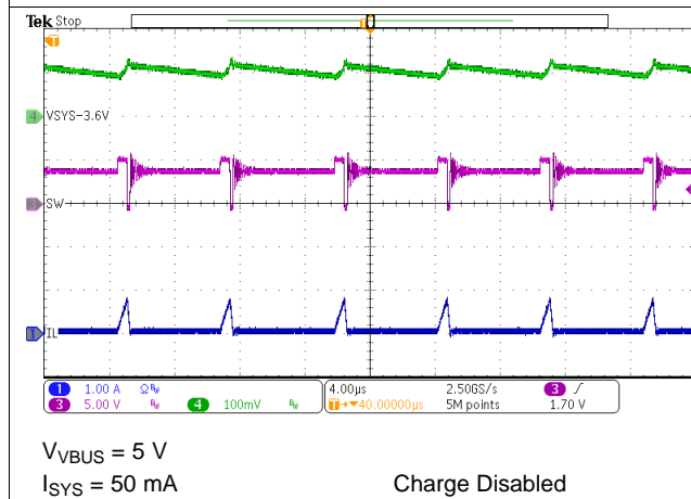
Figure 43. PFM Switching in Buck Mode
