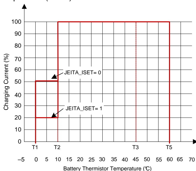
Figure 12. JEITA Profile: Charging Current
