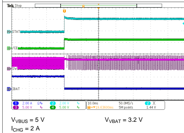
Figure 49. Charge Disable
