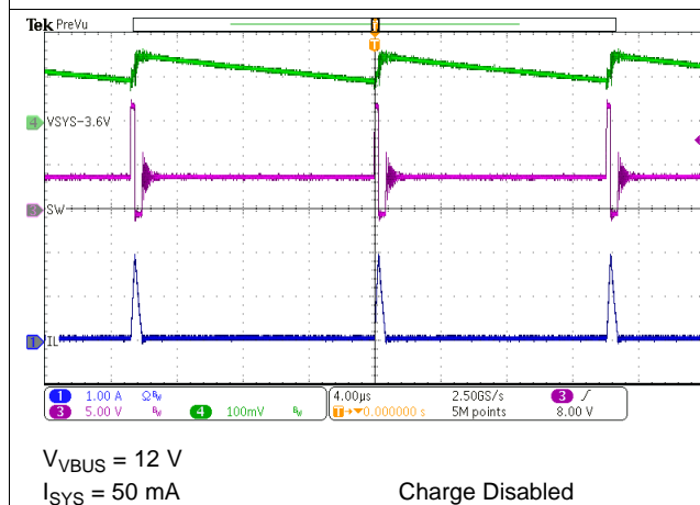
Figure 45. PFM Switching in Buck Mode
