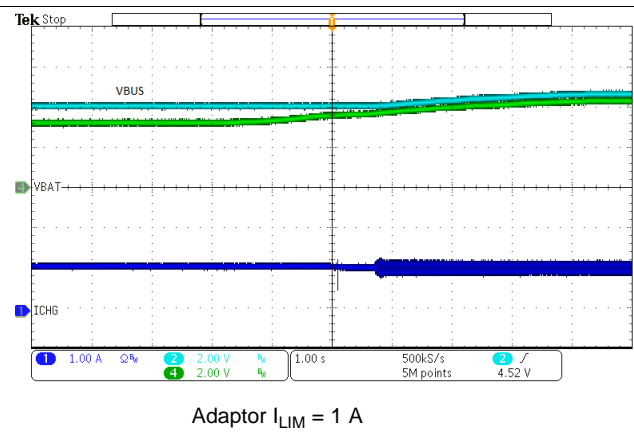
Figure 60. VINDPM Tracking Battery Voltage
