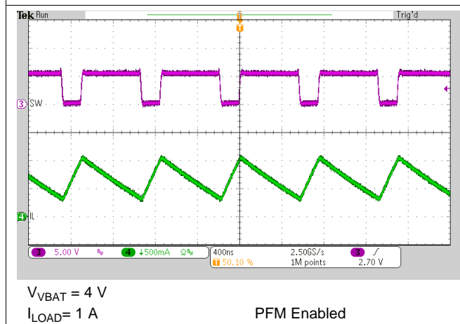
Figure 51. OTG Switching
