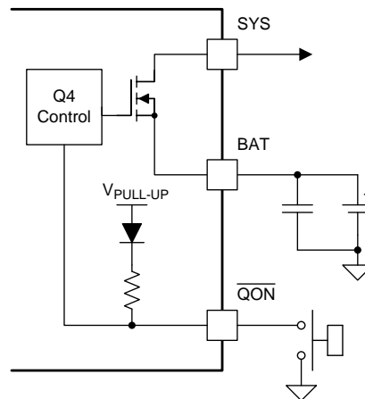
Figure 19. QON Circuit
