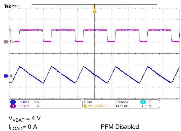
Figure 52. OTG Switching
