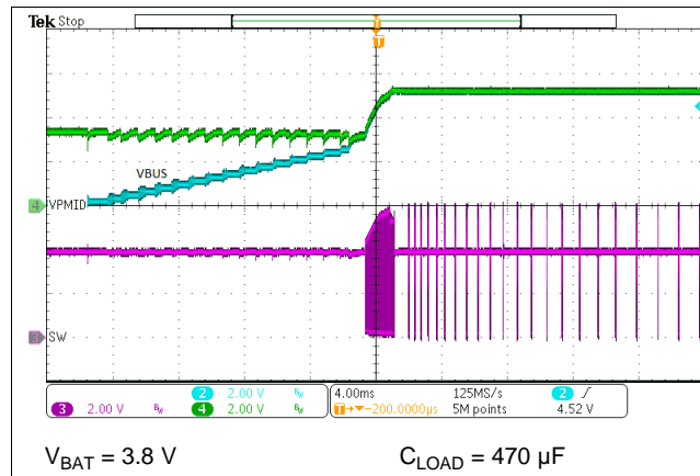
Figure 59. OTG Start-Up
