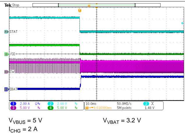
Figure 48. Charge Enable
