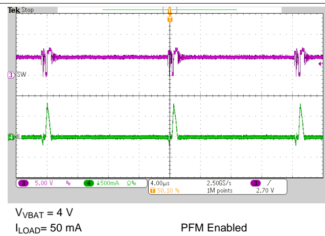
Figure 50. OTG Switching
