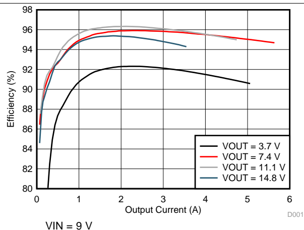
Figure 5. System Efficiency
