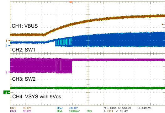
Figure 51. System Regulation
