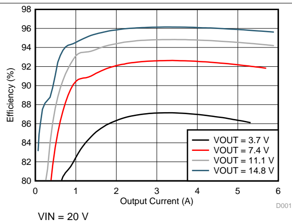
Figure 7. System Efficiency
