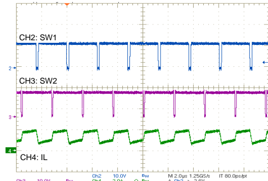
Figure 55. Switching During Buck Boost Mode
