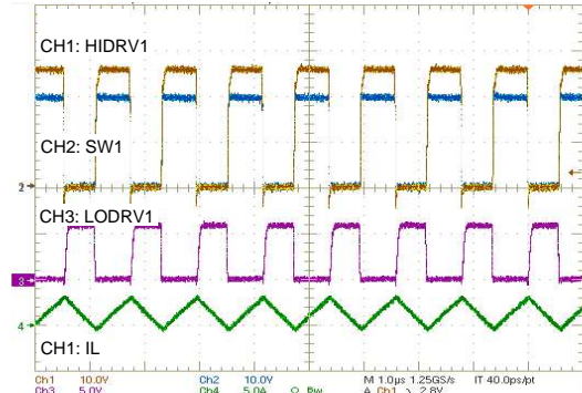
Figure 51. System Regulation
