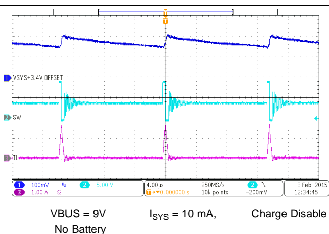
Figure 55. PFM Switching Waveform
