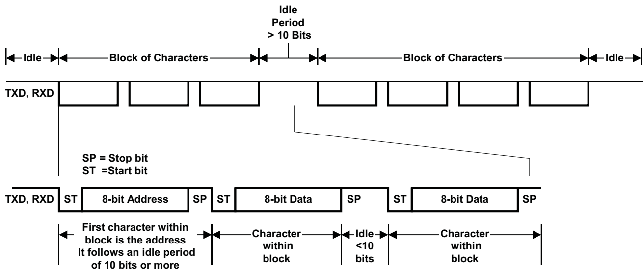
Figure 5. Multi-Drop Operation
