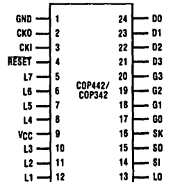
Dual-In-Line Package
