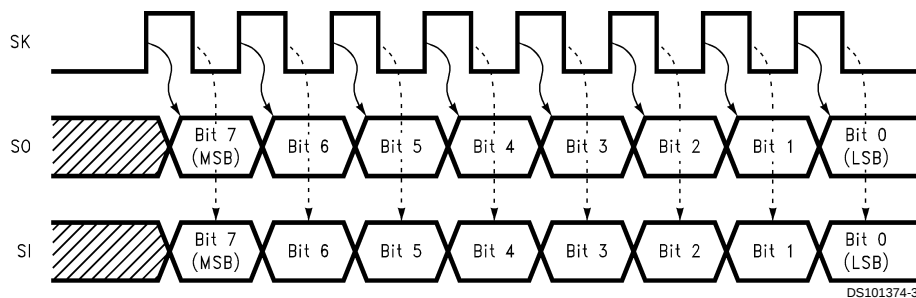
FIGURE 33. MICROWIRE/PLUS SPI Mode Interface Timing, Alternate SK Mode, SK Idle Phase being Low
