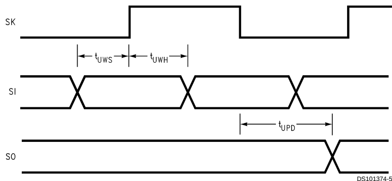
FIGURE 2. MICROWIRE/PLUS Timing
