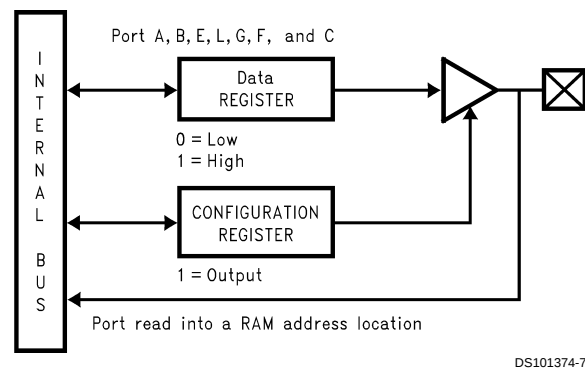
FIGURE 4. I/O Port Configurations—Output Mode
