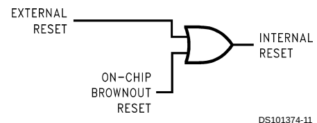
FIGURE 8. Reset Logic
