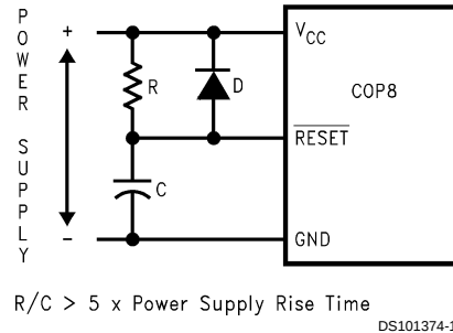
FIGURE 9. Reset Circuit Using External Reset
