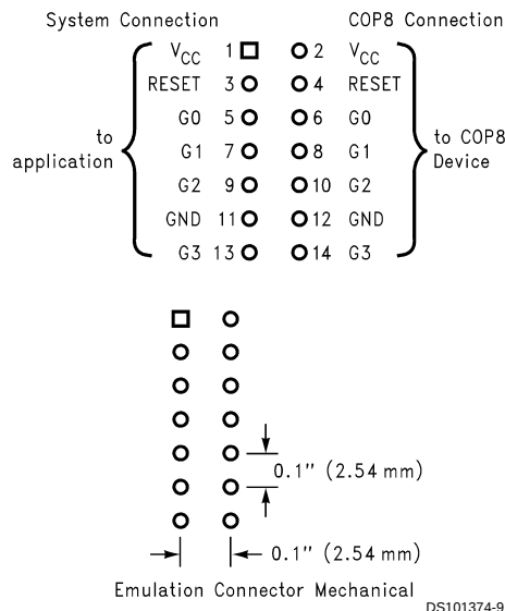
FIGURE 6. Emulation Connection
