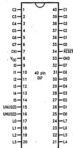
Top View
