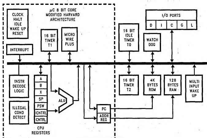
FIGURE 1. Block Diagram
