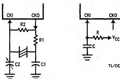
FIGURE 5. Crystal and R/C Oscillator Diagrams
