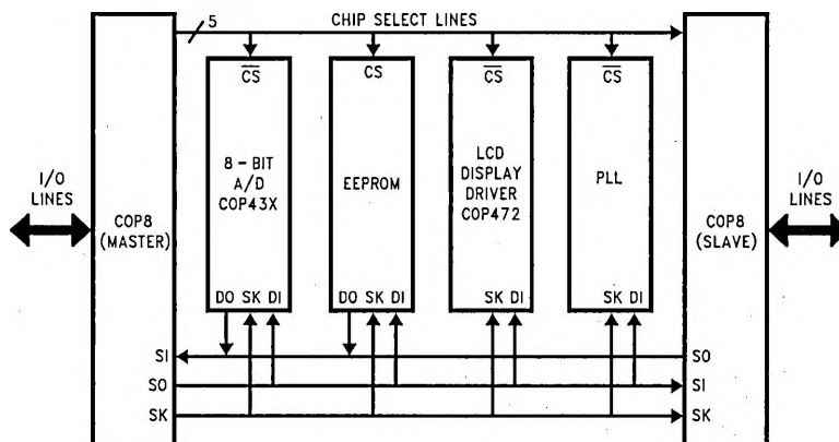
FIGURE 13. MICROWIRE/PLUS Application
