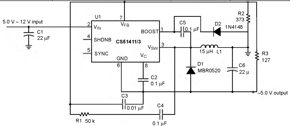
Figure 16. Additional Application Diagram, 5.0 V – 12 V to –5.0 V/400 mA Inverting Converter
