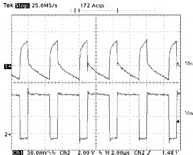
Figure 10. Input Voltage Ripple in a Buck Converter
