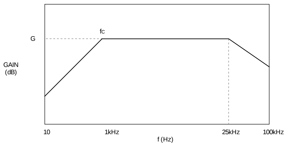
Fig. 2 Frequency Response
