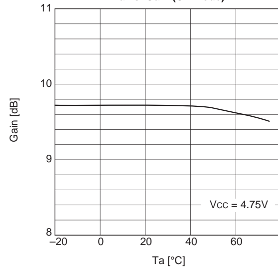
Ta vs. Gain (CL mode)
