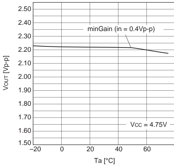
Ta vs. Vout (camera mode)
