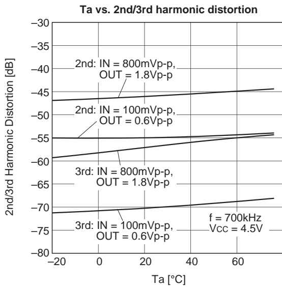
CL mode 2nd/3rd harmonic distortion temperature characteristics
