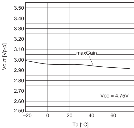
Ta vs. Vout (CL mode)
