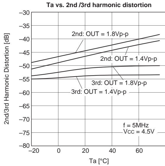
CH mode 2nd/3rd harmonic distortion temperature characteristics
