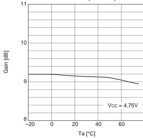
Ta vs. Gain (CH mode)
