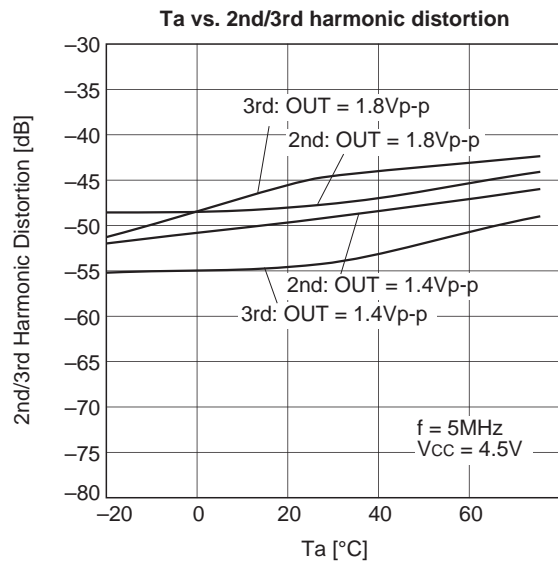
LIN mode 2nd/3rd harmonic distortion temperature characteristics
