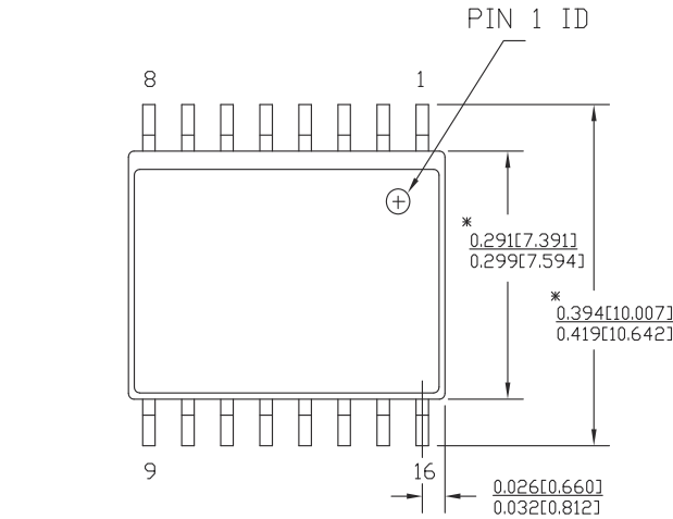
Figure 45. 16-pin SOIC (0.413 × 0.299 × 0.0932) Inches Package Outline, 51-85022
