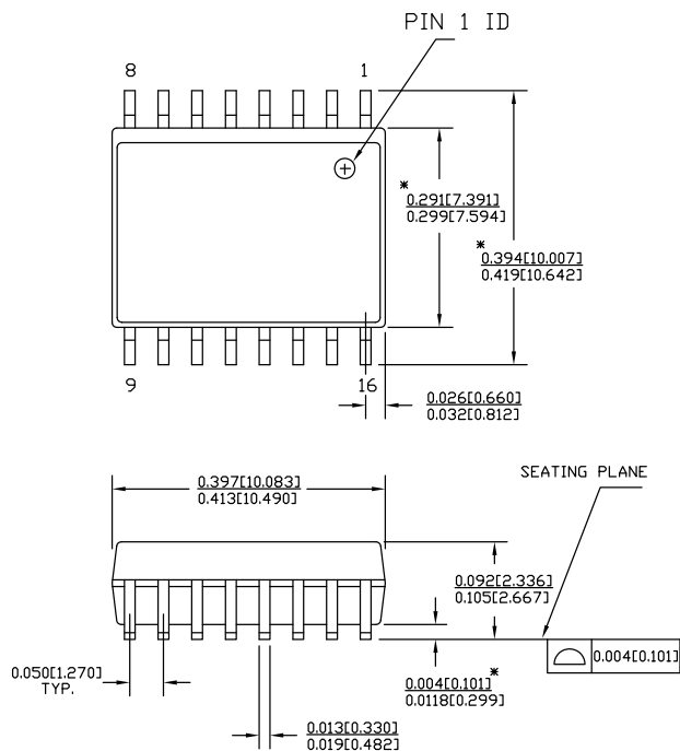
Figure 30. 16-pin SOIC (0.413 × 0.299 × 0.0932 inches) Package Outline, 51-85022
