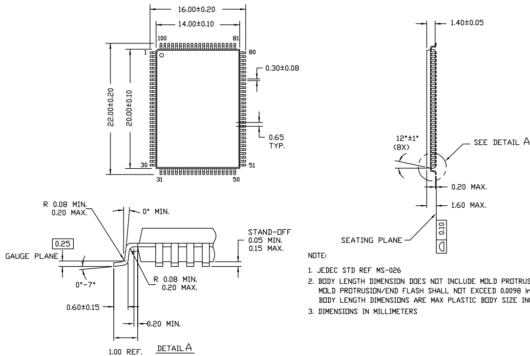
Figure 9. 100-pin TQFP (14 × 20 × 1.4 mm) A100RA Package Outline, 51-85050
