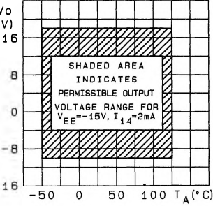
Fig. 7 - Output Voltage Compliance vs Temperature
