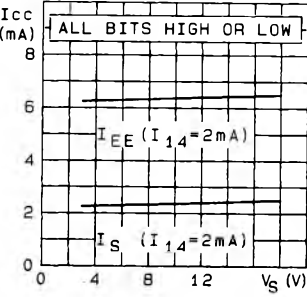
Fig. 3 - Supply Current vs Supply Voltage (VS)
