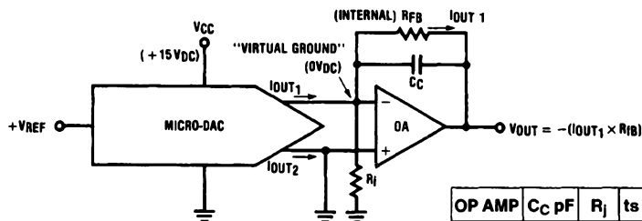
FIGURE 2. Current Mode Switching
