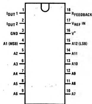
DAC122X Dual-In-Line Package
