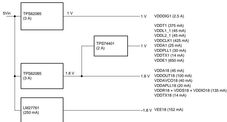
Figure 148. Power Supply Scheme for DAC38RF82 (DAC38RF89)
