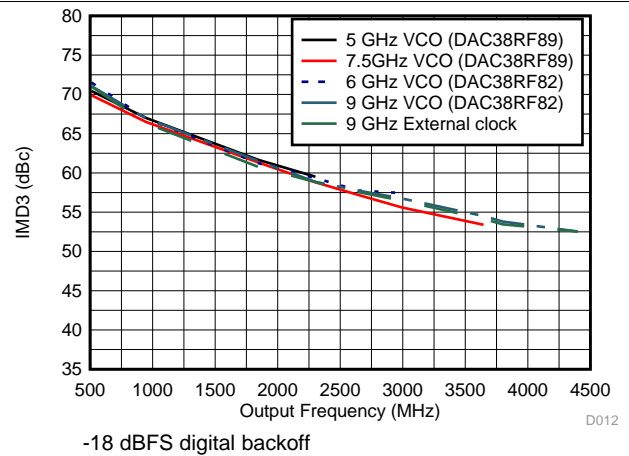
Figure 14. IMD3 vs Output Frequency Over Clocking Option
