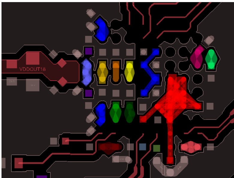
Figure 150. Bypass Capacitors Placed on the Power Supply Pin With In-pad Vias
