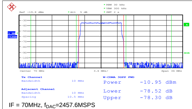
Figure 49. 10-MHz Single Carrier LTE Test Mode 3.1
