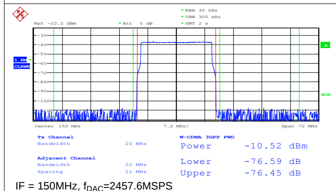
Figure 53. 20-MHz Single Carrier LTE Test Mode 3.1
