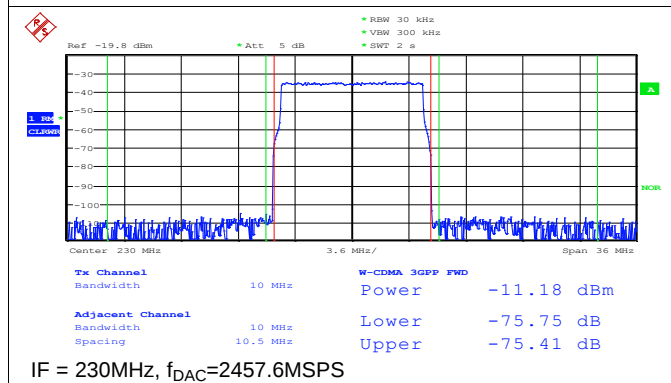
Figure 51. 10-MHz Single Carrier LTE Test Mode 3.1
