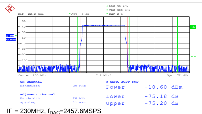
Figure 54. 20-MHz Single Carrier LTE Test Mode 3.1
