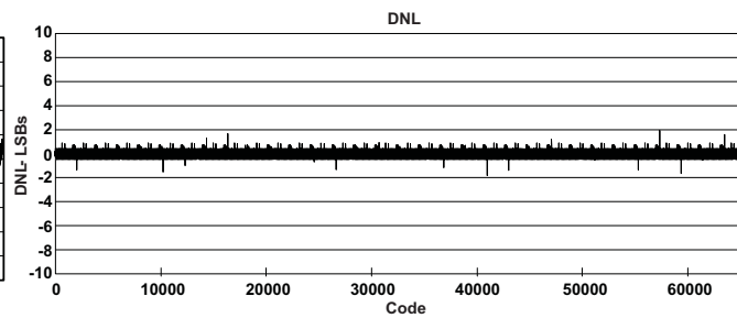
Figure 2. Differential Nonlinearity
