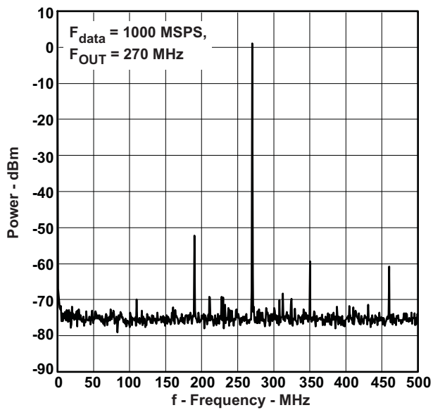
Figure 6. Single-Tone Spectral Plot
