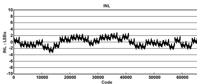
Figure 1. Integral Nonlinearity
