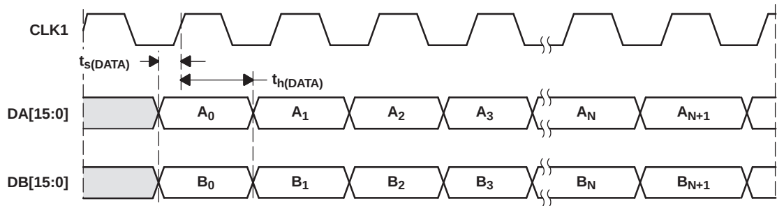
Figure 45. Dual-Bus Mode Timing Diagram (PLL Mode)
